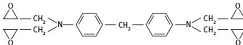
Figure 4: Tetraglycidyl Methylene Dianiline (TGMDA).
