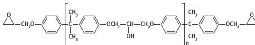
Figure 3: Di-functional epoxy resin.
