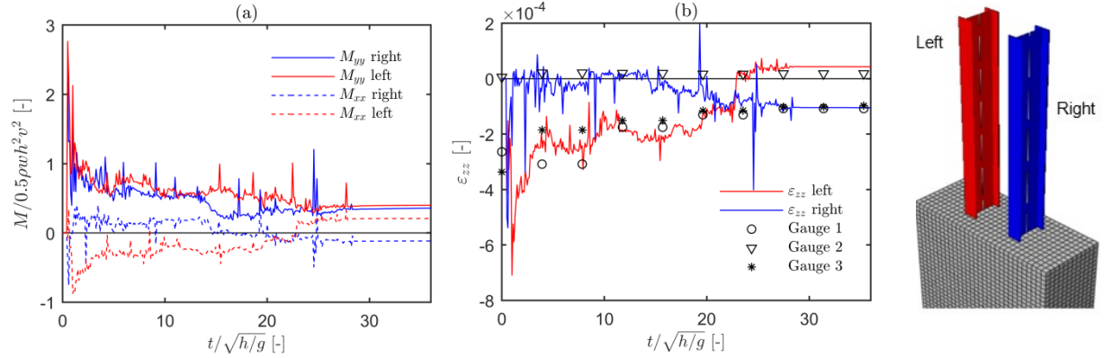
Fig. 5. Time-history of (a) the bending moment registered at the beam junction with the concrete basement, and (b) corresponding strains registered at the location where the strain gauges are installed.
