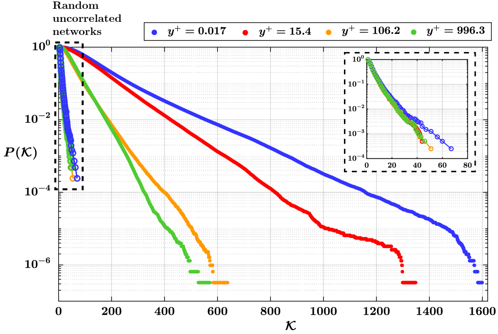
Figure 5.6: Cumulative degree distributions, P(\mathcal{K}) , for the u -based visibility network, averaged over the homogeneous directions. The distributions close to the vertical axis (highlighted in the inset) correspond to networks built on shuffled time-series (similar colours refers to similar y^+ values). The slopes of the distributions are (-1.01, -1.08, -2.85, -2.86) \cdot 10^{-2} from y^+ = 0.017 to y^+ = 996.3 , respectively; the slope for the shuffled series is about 2 \cdot 10^{-1} . The coefficient of determination, R^2 , of the fittings is always above 0.99.
