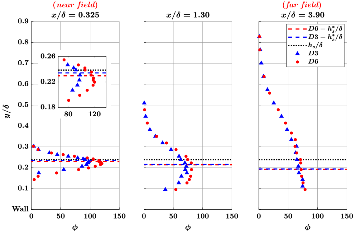
Figure 5.20: Vertical profiles of the average peak occurrence \phi [Hz] based on signals of v'c' . The profiles are plotted in the near field and in the far field, for D3 (blue marker) and D6 (red marker). The source axis height, h_s , is illustrated as a horizontal dotted line, while the plume axis height, h_s^* , is displayed as a blue (red) dashed line for the source D3 (D6). The inset at x/\delta = 0.325 shows a zoom around the plume axis.
