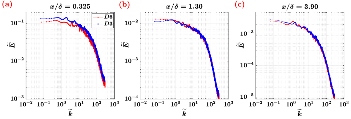
Figure 5.16: Normalized spectral density, \langle \tilde{E} \rangle , as a function of the normalized wavenumber, \tilde{k} , of the wall-normal turbulent transport, v'c' . Spectra are evaluated at the source axis ( y = h_s ), for D3 and D6, at three streamwise locations: (a) in the near field ( x/\delta = 0.325 ), (b) at an intermediate location ( x/\delta = 1.30 ), and (c) in the far field ( x/\delta = 3.90 ).
