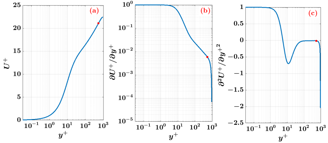
Figure B.2: Wall-normal profiles in wall-units of (a) the mean velocity, U^+ , (b) the first derivative of U^+ (i.e., the mean shear), and (c) the second derivative of U^+ . The red points highlight the value of each quantity at y^+ \approx 530 .
