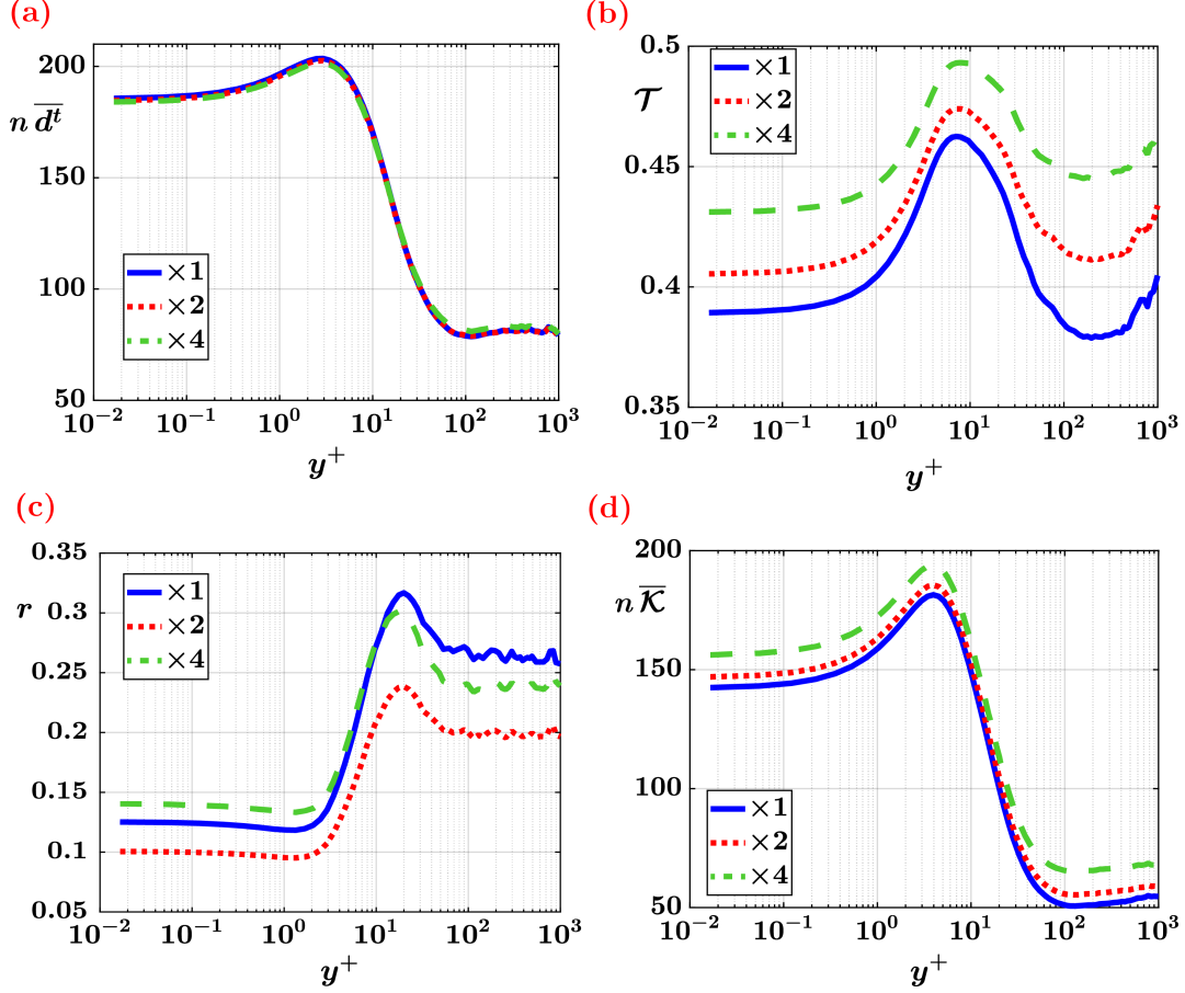
Figure 5.9: Averaged metric behaviours as function of y^+ for three different time samplings of the streamwise velocity time-series, u . The curves are obtained with n\Delta t , where the sampling is n = 1 (blue), n = 2 (red), n = 4 (green).
