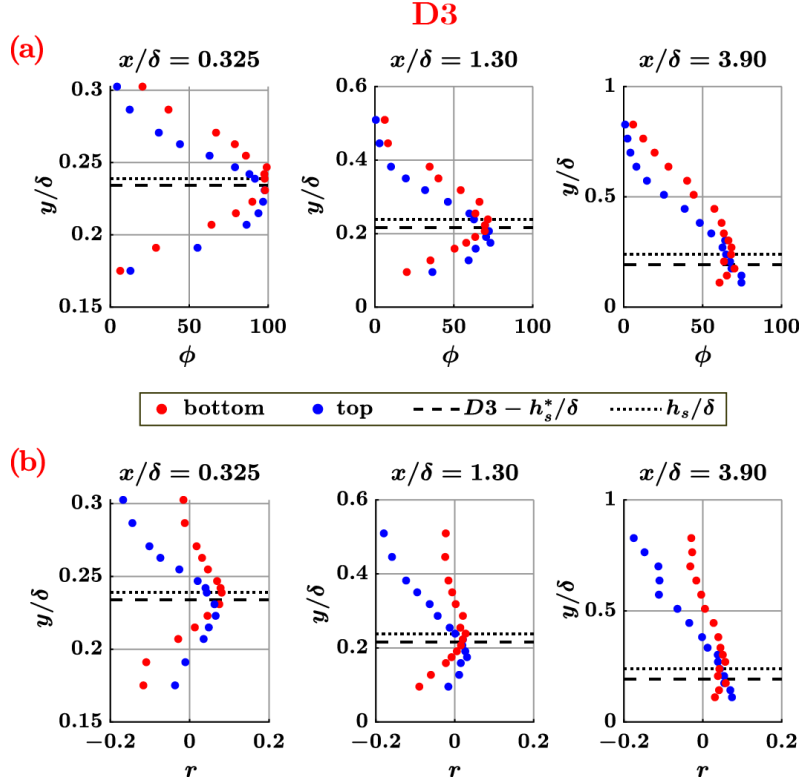
Figure 5.23: Vertical profiles of (a) the average peak occurrence, \phi , and (b) the assortativity coefficient, r , for the top- and bottom-visibility in the configuration D3. The source axis height, h_s , is illustrated as a horizontal dotted line, while the plume axis height, h_s^* , is displayed as a dashed horizontal line for both D3 and D6.
