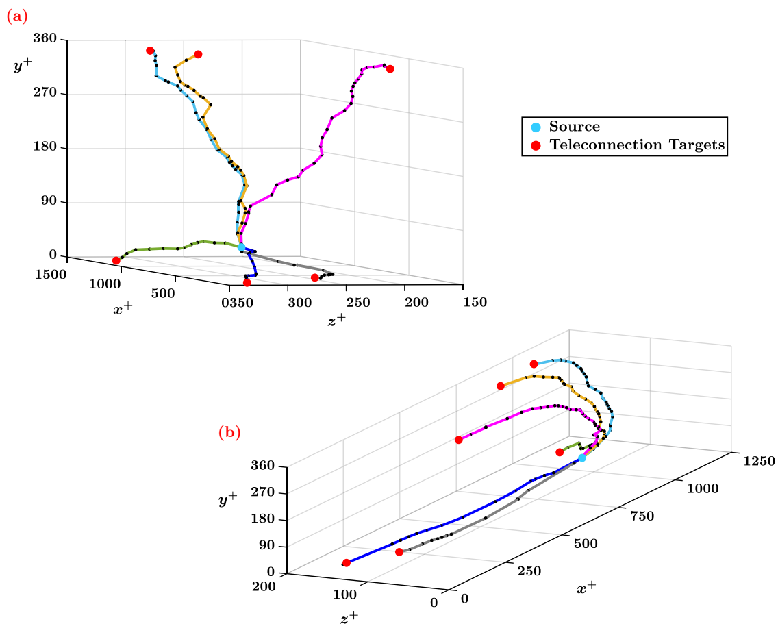
Figure 6.16: Example of shortest paths between a source-node close to the wall (light-blue dot) and six teleconnected neighbours of it, shown through two 3D views. Different colors refer to different targets, while black points indicate intermediate nodes in the paths.
