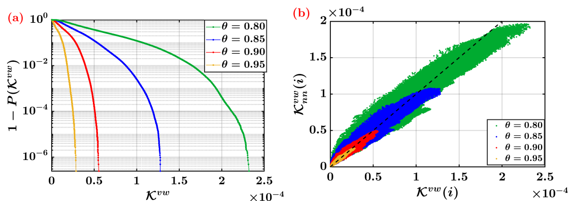
Figure 6.23: Network built on the wall-normal velocity, v . (a) Cumulative \mathcal{K}^{vw} distribution and (b) weighted average nearest neighbours assortativity measure, \mathcal{K}_{nm}^{vw}(i) , as a function of \mathcal{K}^{vw} , for different thresholds \theta .
