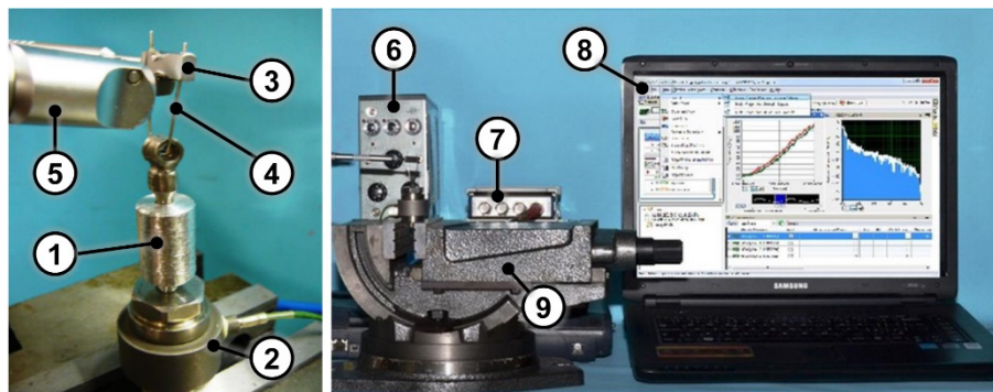
Figure 1. (Left) Close up view of the test setup with the cylindrical aluminum support (1), the load cell (2), the loop holder (3), the loop (4) and the CoronaFlex® (5); (Right) Test setup composed of the amplifier (6), the data acquisition board (7), the laptop equipped with LabVIEW SignalExpress (8) and the vise (9).
