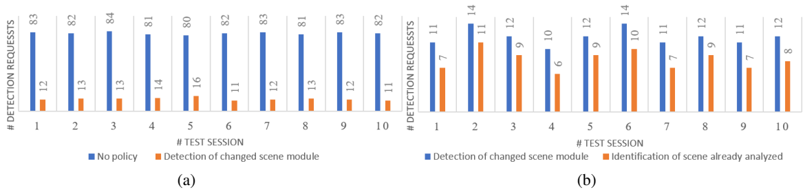
Figure 5: (a.) Detection requests reduction related to the "Detection of changes in current scene" (Fig.1, F) module; (b.) Detection requests reduction related to the "Identification of scene already analyzed" (Fig.1, I) module.
