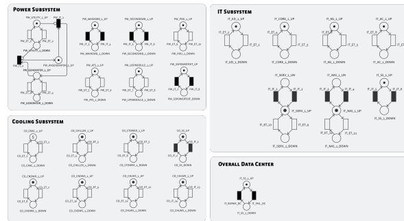
Figure 1. Tier I data center SPN model (from [16])
