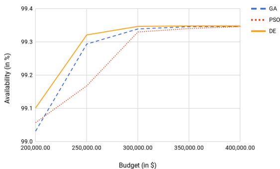
Figure 5. Availability found by optimization algorithms
