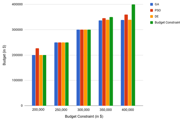
Figure 4. Budget estimated by optimization algorithms
