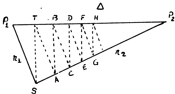
Fig. 1 — Geometric configuration of the three-body problem at some arbitrary time t . ST , BA , CD , EF , ... are perpendicular to the side \Delta . AT , CB , ED , GF , ... are the corresponding parallels to the side r_1 .
