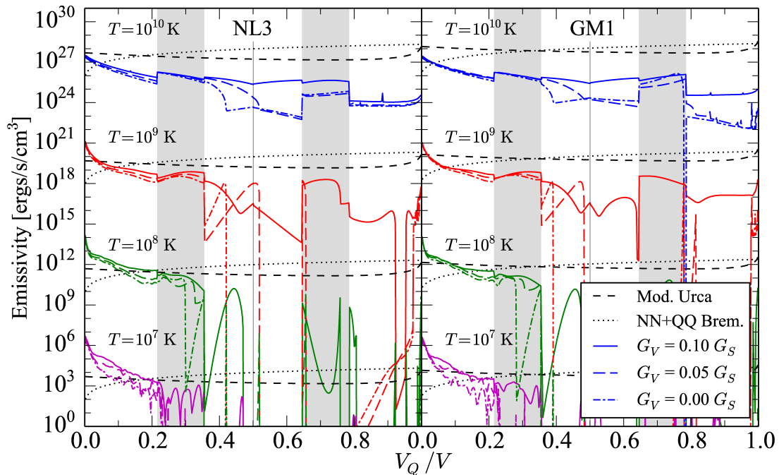
Fig. 10. (Color online) Comparison of the neutrino emissivity due to electron-lattice interactions in the quark-hadron mixed phase to modified Urca and bremsstrahlung (NN+QQ) processes in the mixed phase for different parameterizations. Shading represents geometric structures as shown in Figure 3.
