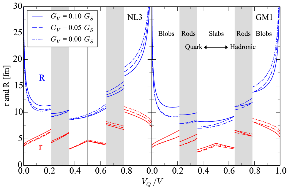
Fig. 3. (Color online) Rare phase structure radius r and Wigner-Seitz cell radius R plotted against quark fraction for the given parameterizations and vector coupling constant values. The change in background color refers to a change in structure as shown in the right panel. Discontinuities in the radii are also associated with changes in the crystalline structure.
