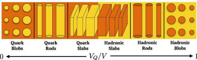
Fig. 2. (Color online) Spherical blob, rod, and slab rare phase structures. V_Q/V_{\text{Total}} denotes the quark fraction of the mixed phase.
