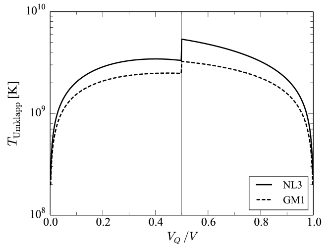
Fig. 5. Temperature below which Umklapp processes are frozen out ( T_{\text{Umklapp}} ) as a function of quark fraction, and contributions to the neutrino emissivity due to electron-phonon interactions become negligible.
