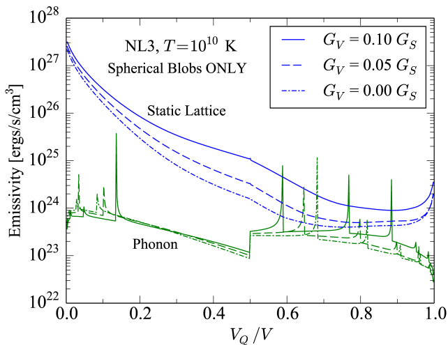
Fig. 9. (Color online) Comparison of the static lattice and phonon contributions to the neutrino emissivity for the NL3 parameter set at T > T_{\text{Umklapp}} . The comparison is performed for only the spherical blob geometry, as the phonon contribution is not determined for other geometries.
