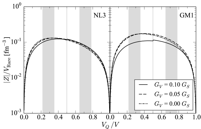
Fig. 4. (Color online) Rare phase structure charge number per unit volume plotted against quark fraction for the given parameterizations and vector coupling constant values. Slight discontinuity at \chi = 0.5 is due to a higher number of positively charged baryons (electrons make up difference in negative charge).
