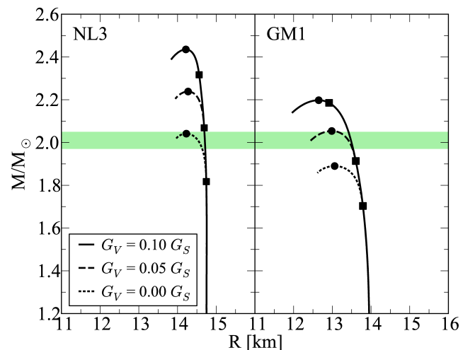
Fig. 6. (Color online) Mass-radius relationship of neutron stars for the given parameterizations and vector coupling constant values listed in Table 1. Square markers indicate the beginning of the quark-hadron mixed phase, and dot markers indicate the location of the maximum mass. The green shaded region indicates the mass constraint set by PSR J3048+0432.
