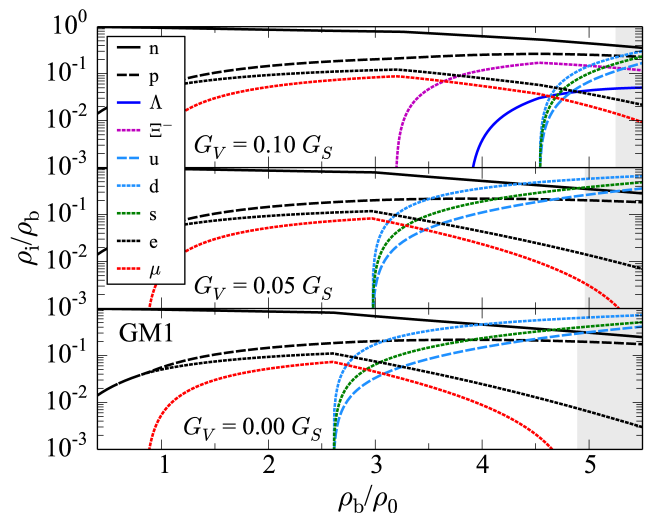
Fig. 8. (Color online) Same as Figure 7 but for the GM1 parameterization.
