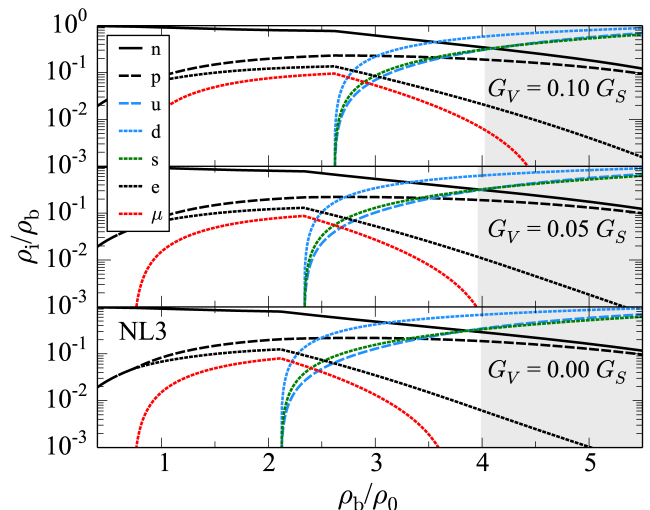
Fig. 7. (Color online) Relative particle number densities as a function of baryonic density (in units of nuclear saturation density) for the NL3 parameterization and given values of the vector coupling constant. Grey shaded region indicates the densities beyond the maximum mass neutron star for the given parameterization.
