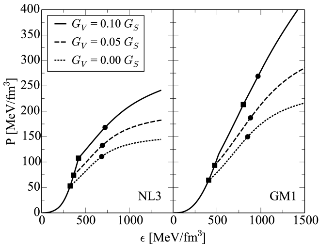
Fig. 1. Equations of state of this work. Shown are the hadronic and mixed phases. Square markers indicate the beginning of the quark-hadron mixed phase, and dot markers indicate the location of the maximum mass.
