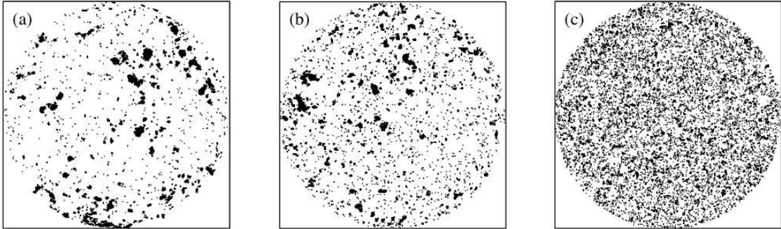
Figure 2: Typical snapshot configurations for N = 16384 and different values for \alpha , namely: (a) \alpha = 0.02 , (b) \alpha = 0.093 , and (c) \alpha = 0.20 . These configurations have been generated by applying the algorithm proposed in Ref. [18], in which the O(n) rotational invariance is enforced explicitly in the model's dynamic rules.
