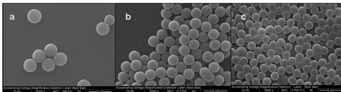
Figure 1. SEM micrographs (5000X) of polystyrene spheres prepared using ACVA as polymerization initiator and different PVP to styrene ratios: a) 1, b) 3, c) 10% (w/w). Bar: 5 \mu m.
