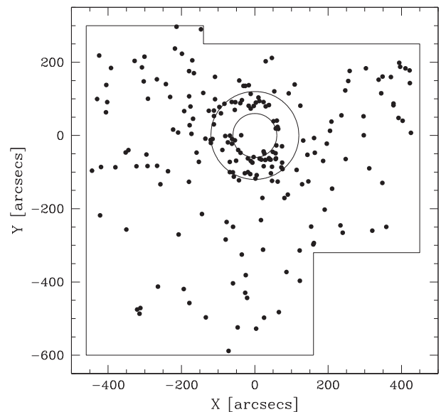
Figure 23. Distribution on the sky of 229 objects with g'_0 from 23.5 to 25 and (g-i)'_0 from 0.30 to 0.75. The reference circles have 60–120 arcsec radius.
