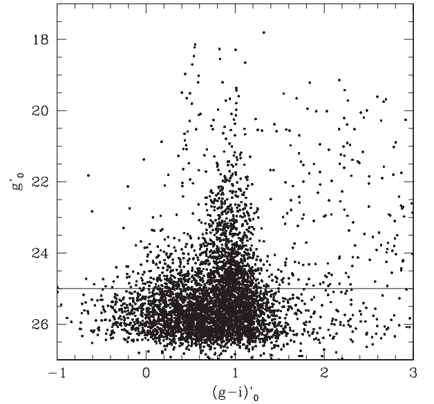
Figure 5. g'_0 versus (g-i)'_0 colour–magnitude diagram for the unresolved sources (4856 objects). The horizontal line at g'_0 = 25.0 indicates the limiting magnitude of the analysis presented in this work.
