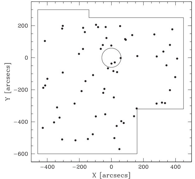
Figure 22. Distribution on the sky of 66 objects brighter than g = 23.50 and (g-i)'_0 colours between 0.30 and 0.75. The reference circle, centred on the galaxy nucleus, has a 60 arcsec radius.
