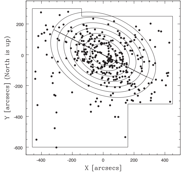
Figure 26. Distribution on the sky of 340 objects brighter than g'_0 = 25 and (g - i)_0 = 0.90\text{--}1.05 (‘intermediate’ GCs). The ellipses (from a = 90 to 360 arcsec) have a flattening q = b/a = 0.70 . The ellipses have a PA of 63 deg.
