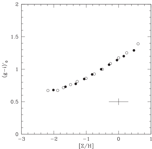
Figure 17. Chemical abundance [Z/H] versus (g-i)'_0 colour relation based on the Usher et al. (2012) calibration (filled dots) compared with the 12 Gyr PARSEC model including a correction to the g' magnitude described in the text. The cross shows typical errors for each data point.
