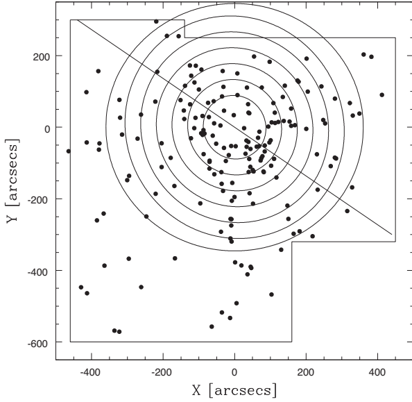
Figure 24. Distribution on the sky of 177 objects brighter than g = 25.0 and (g - i)_0 colours between 0.75 and 0.90 (‘blue’ GCs). The ellipses (from a = 90 to 360 arcsec) have a flattening q = b/a = 0.96 . The straight line indicates the position of the major axis of the galaxy.
