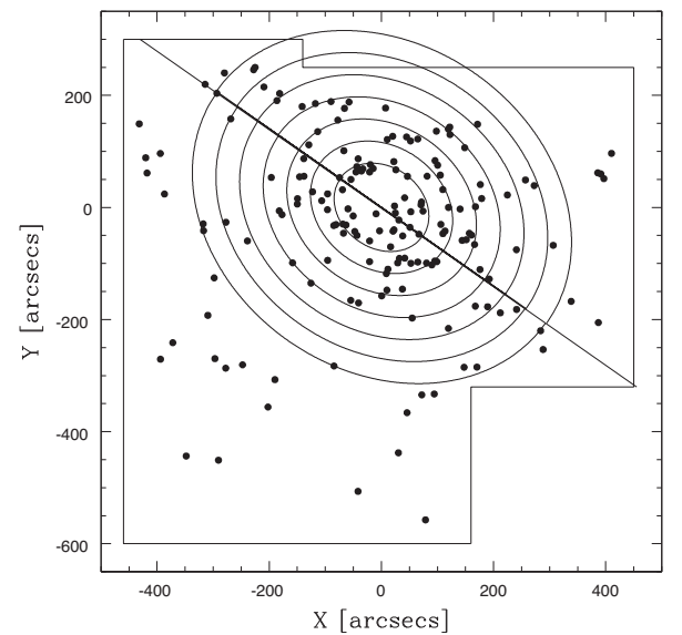
Figure 27. Distribution on the sky of 170 red GC candidates brighter than g'_0 = 25 and (g - i)_0 = 1.05\text{--}1.35 (‘red’ GCs). The ellipses (from a = 90 to 360 arcsec) have a flattening q = b/a = 0.81 . The straight line indicates the position of the major axis of the galaxy.
