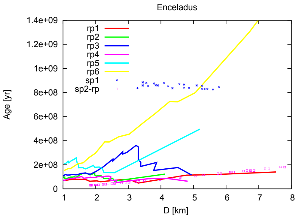
Figure 11: Age of the rp surfaces of Enceladus with respect to D.
