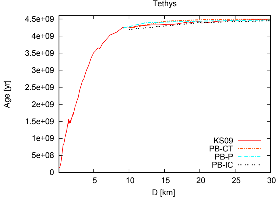
Figure 6: Age of the Ithaca Chasma (PB-IC) interior terrain, plain units (PB-CT) and (PB-P) from Voyager images and Cassini images (KS09) of Tethys with respect to D .
