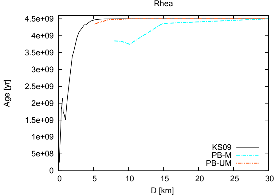
Figure 8: Age of equatorial mantled (PB-M) and unmantled regions (PB-UM) from Voyager images and Cassini images (KS09) of Rhea with respect to D .
