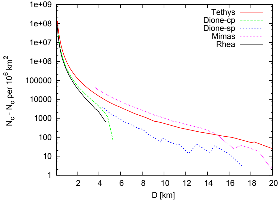
Figure 2: Difference between the cumulative number of theoretical craters and observed craters for Tethys, Dione, Mimas and Rhea according to D .
