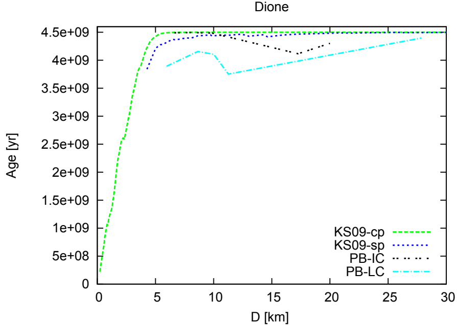
Figure 7: Age of an intermediate crater plains unit (PB-IC) and a smooth plains unit (PB-LC) from Voyager images and cratered plains (cp) and smooth plains (sp) from Cassini images (KS09) of Dione with respect to D .
