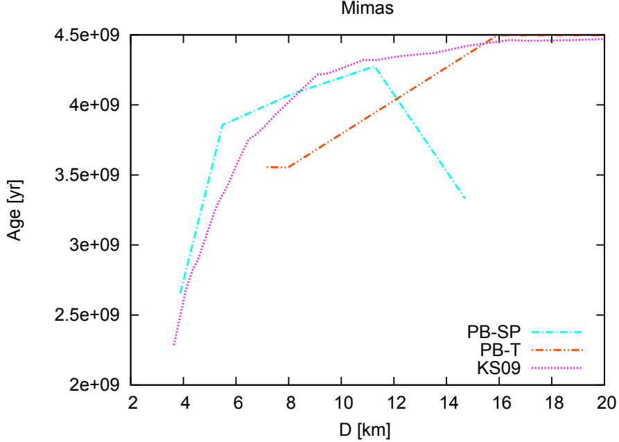
Figure 5: Age of the south polar (PB-SP) and intermediate latitudes regions (PB-T) from Voyager and Cassini images (KS09) of Mimas with respect to D .
