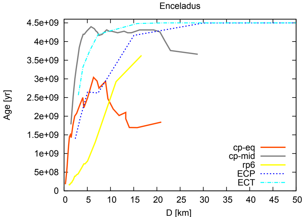
Figure 10: Age of the cp and rp6 surfaces of Enceladus with respect to D .
