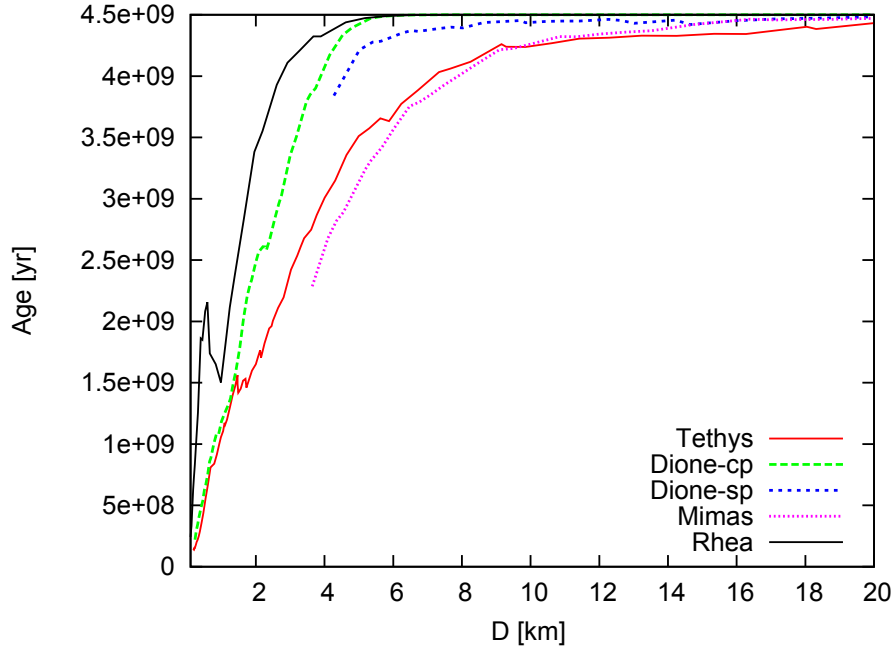
Figure 3: Age of the surface of Tethys, Dione, Mimas and Rhea according to D.
