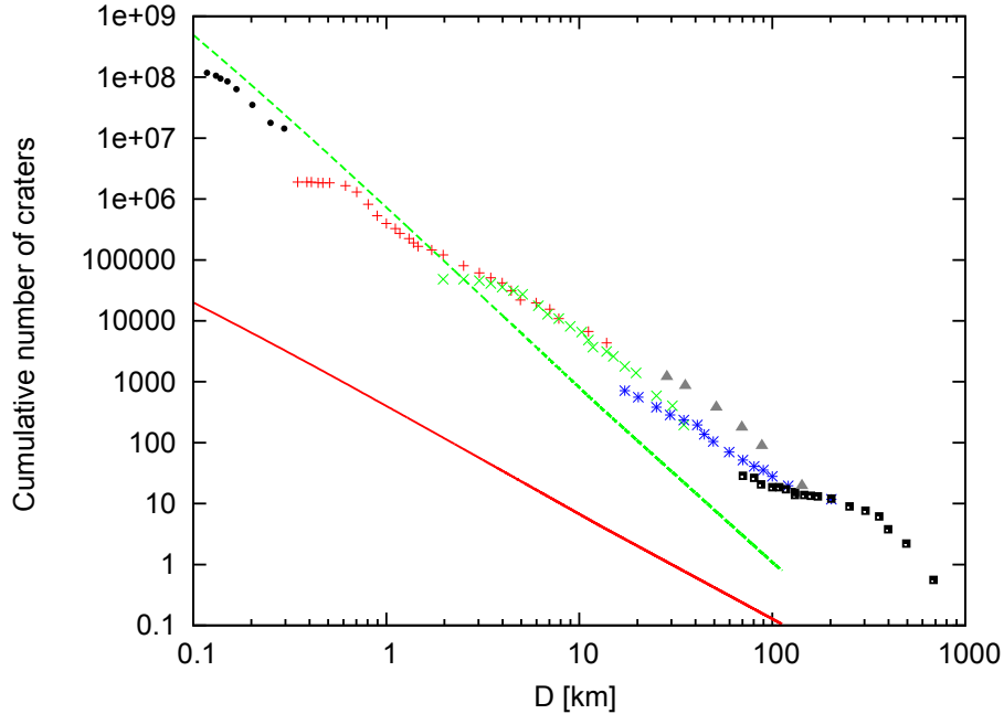
Figure 4: Cumulative number of craters of Iapetus with respect to D . Points represent the number of craters obtained by Denk et al. (2010) and Plescia and Boyce (1983) (the gray ones), the red curve represents the cumulative number of craters obtained by our model for s_2 = 2.5 , and the green one for s_2 = 3.5 .
