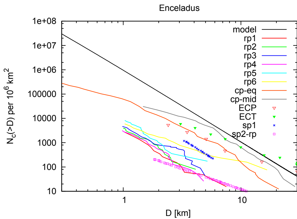
Figure 9: Cumulative number of craters calculated from model by DZ13 ( s_2 = 3.5 ) and crater counts from Voyager (ECP, ECT, sp1, sp2-rp) and from Cassini by KS09.
