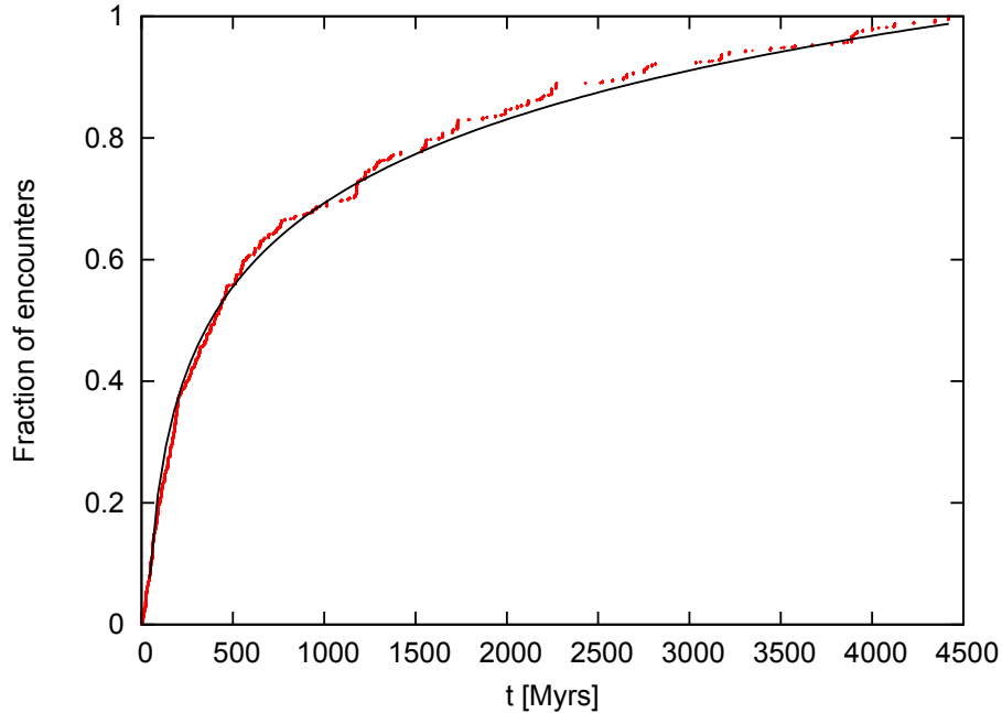
Figure 1: Fraction of encounters of SDOs with Saturn versus time and the fit to the data.
