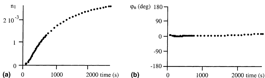
Fig. 2. Time dependence of the gratings written at normal incidence, 532 nm, 6 mW/cm 2 . (a) Modulation n_1 of the refractive index; (b) phase shift \varphi_n of the index grating.
