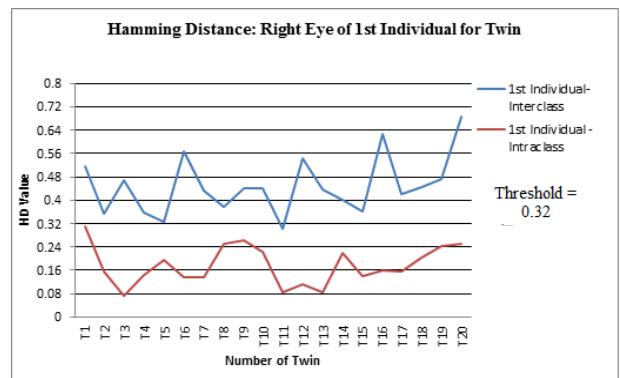
Fig. 5 Hamming distance value for right eyes of the first individual in twin
