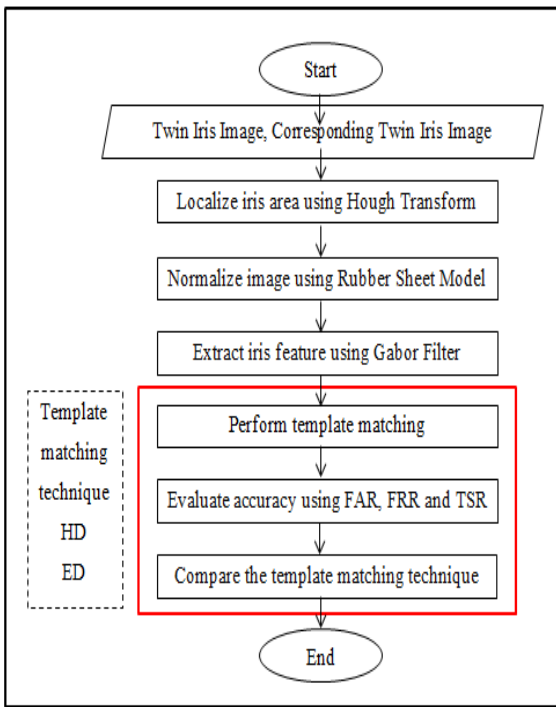
Fig. 1 Flowchart for twin iris recognition
