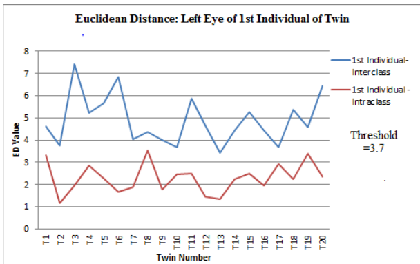
Fig. 7 Euclidean distance value for left eyes of the first individual in twin
