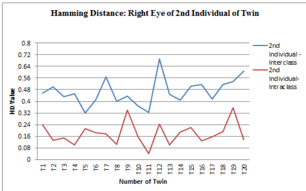
Fig. 6 Hamming distance value for right eyes of the second individual in twin
