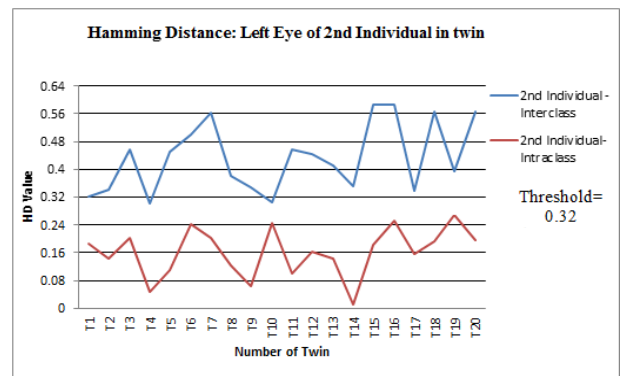
Fig. 4 Hamming distance value for left eyes of the second individual in twin
