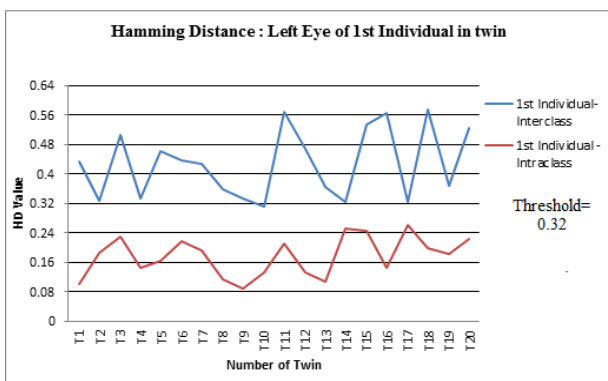
Fig. 3 Hamming distance value for left eyes of the first individual in twin
