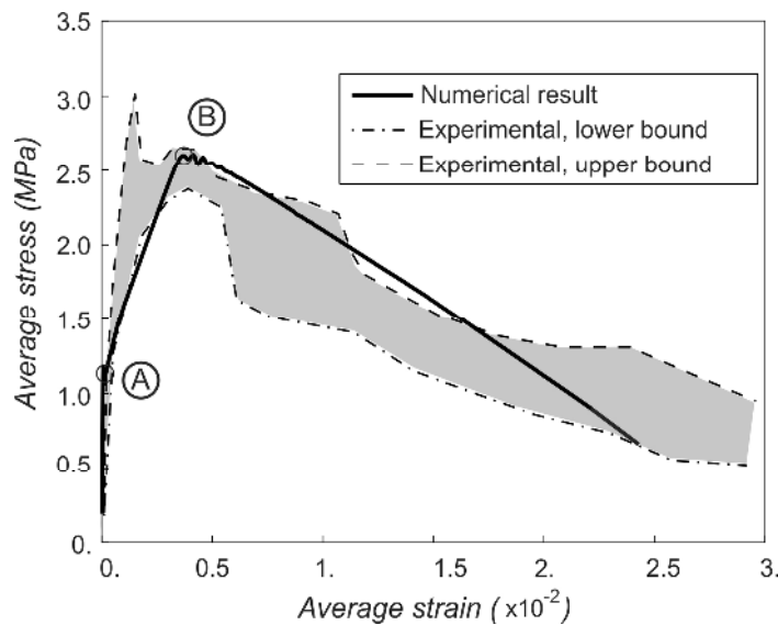
Figure 12. HPRFC dogbone shape specimen subjected to the tensile test. Comparison between experimental and numerical results. Experimental test correspond to the High Strength Hooked Steel fibers case (specimen D-H-H-0.75, pp.80 in Suwannakarn, 2009).
