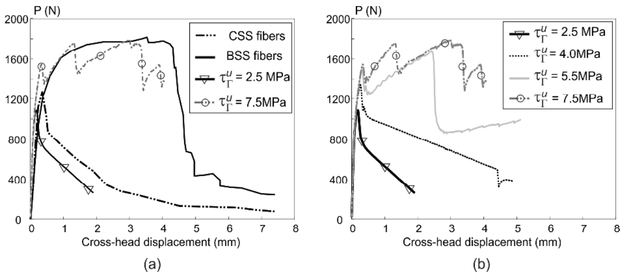
Figure 6. Four-point bending beam test. Load as a function of cross head displacement steel-wire-reinforced cement specimens: a) comparison between experiments and numerical results using the material parameter: \tau_{\Gamma}^u = 2.5\text{MPa} and \tau_{\Gamma}^u = 7.5\text{MPa} , respectively; b) Load vs. cross head displacement curves for different values of: \tau_{\Gamma}^u .
