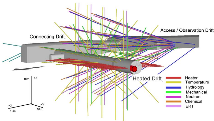
Fig. 1. Three-dimensional view of the Yucca Mountain DST. The color-coded lines indicate boreholes for various measurements of thermally driven THM responses.
