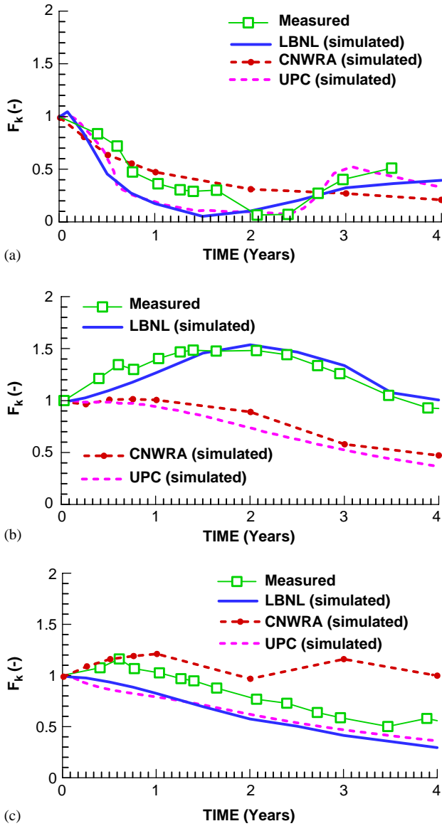
Fig. 11. Measured and simulated evolution of permeability correction factor ( F_k = k/k_i ) for three different borehole sections. (a) Section 76:4; (b) Section 74:4; (c) Section 76:1.
