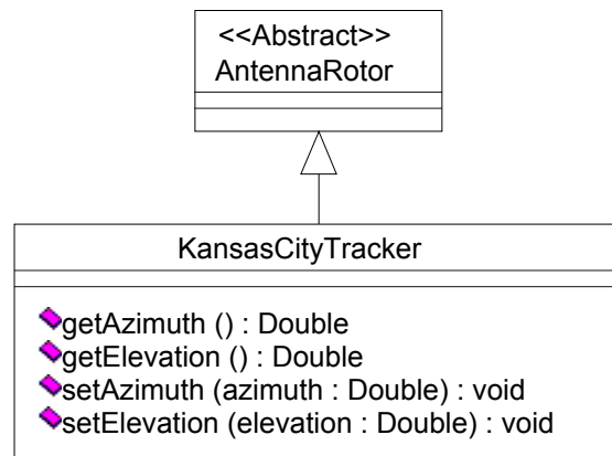
Figure 16. KansasCityTracker Class Definition.
