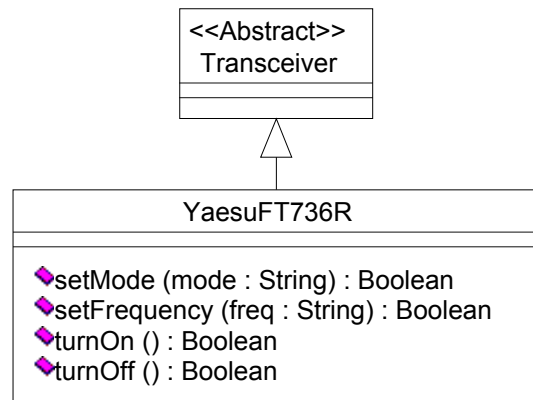
Figure 15. YaesuFT736R Class Definition.
