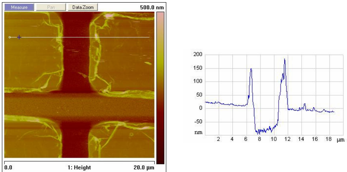
Figure 4.10. Section analyses of 10 \times 10 \mu\text{m}^2 mesas obtained by AFM.
