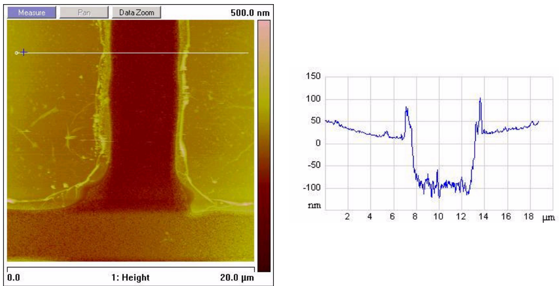
Figure 4.9. Section analyses of 20 \times 20 \mu\text{m}^2 mesas obtained by AFM.
