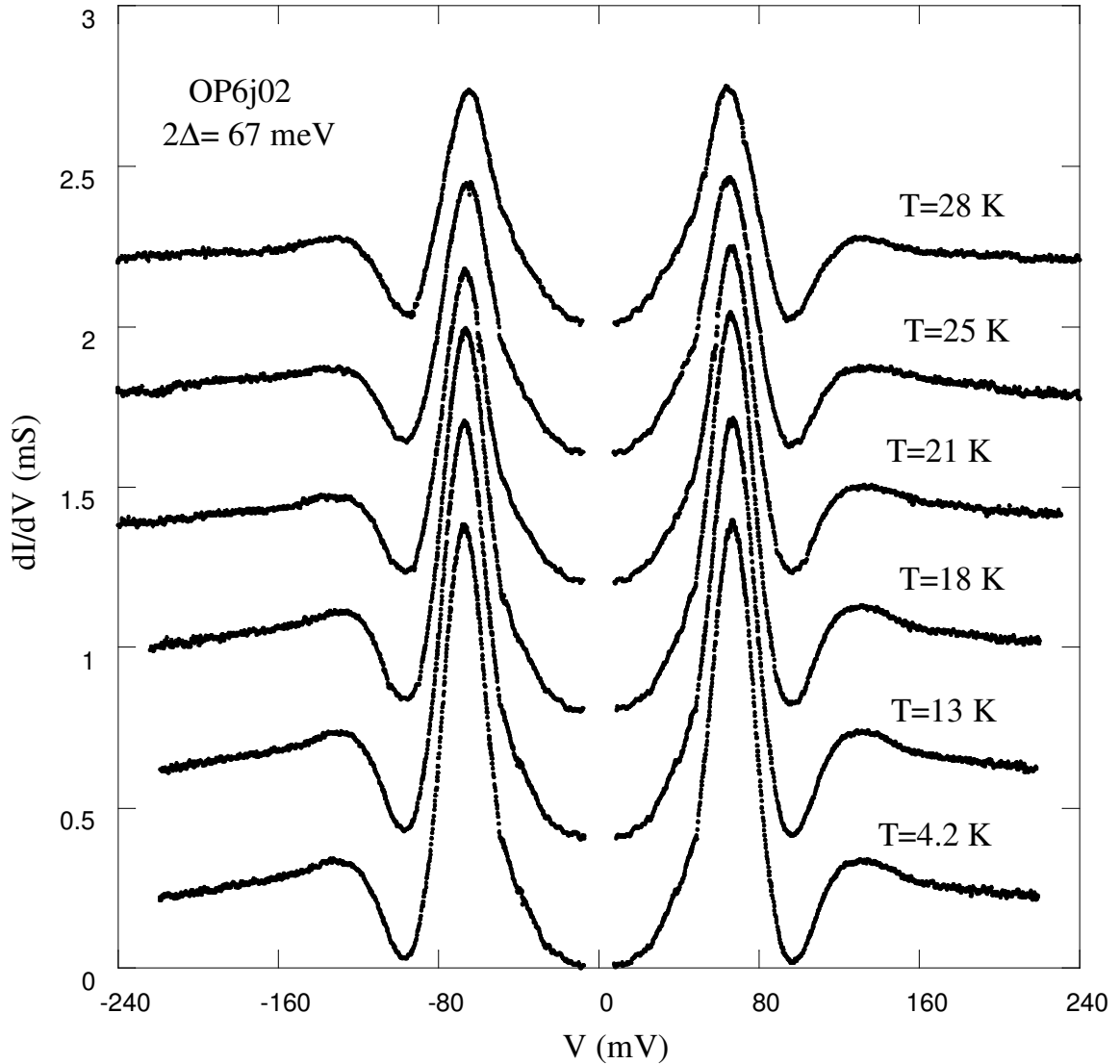
Figure 4.4. Temperature dependence of tunneling conductance characteristics for an SIS junction on nearly optimally doped Bi-2212 (with T_c=92 K).
