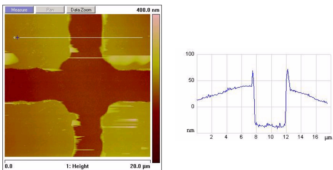
Figure 4.29. The section analyses of the mesas on BH3e
