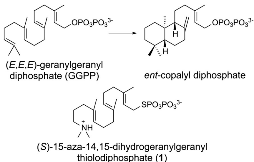
Fig. 1. Cyclization reaction catalyzed by ent -copalyl diphosphate synthase and the unreactive substrate analogue (S)-15-aza-14,15-dihydrogeranylgeranyl thiolodiphosphate (1).
