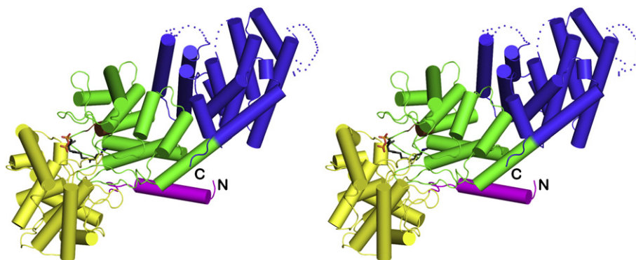
Fig. 2. Overall structure of the CPS-1 complex color-coded as follows: \alpha domain = blue; \beta domain = green; \gamma domain = yellow; N-terminal helix = magenta; DXDD general acid motif = brown. The N- and C-termini are indicated by “N” and “C,” respectively. The \gamma domain is inserted between the N-terminal helix and the second helix of the \beta domain. Inhibitor 1 is shown as a stick figure bound in the active site at the interface of the \beta and \gamma domains.
