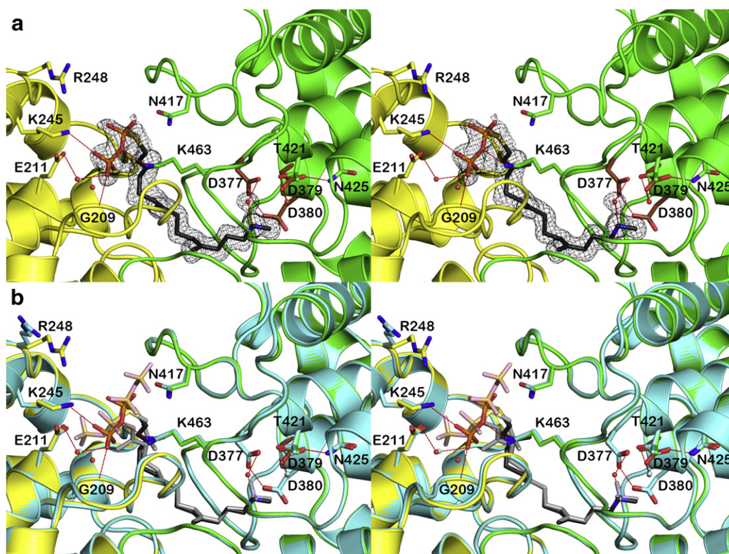
Fig. 3. (a) Simulated annealing omit map (contoured at 4.0\sigma ) of the CPS-1 complex at 1.55 Å resolution. Atoms are color-coded as follows: C = green ( \beta domain), brown (DXDD general acid motif in the \beta domain), or yellow ( \gamma domain), N = blue, O = red, P = orange, S = yellow; selected water molecules are shown as small red spheres, and hydrogen bond interactions are indicated by dash red lines. (b) Superposition of the 1.55 Å-resolution structure of the CPS-1 complex color-coded as in (a) with the 2.25 Å-resolution structure (all atoms cyan).
