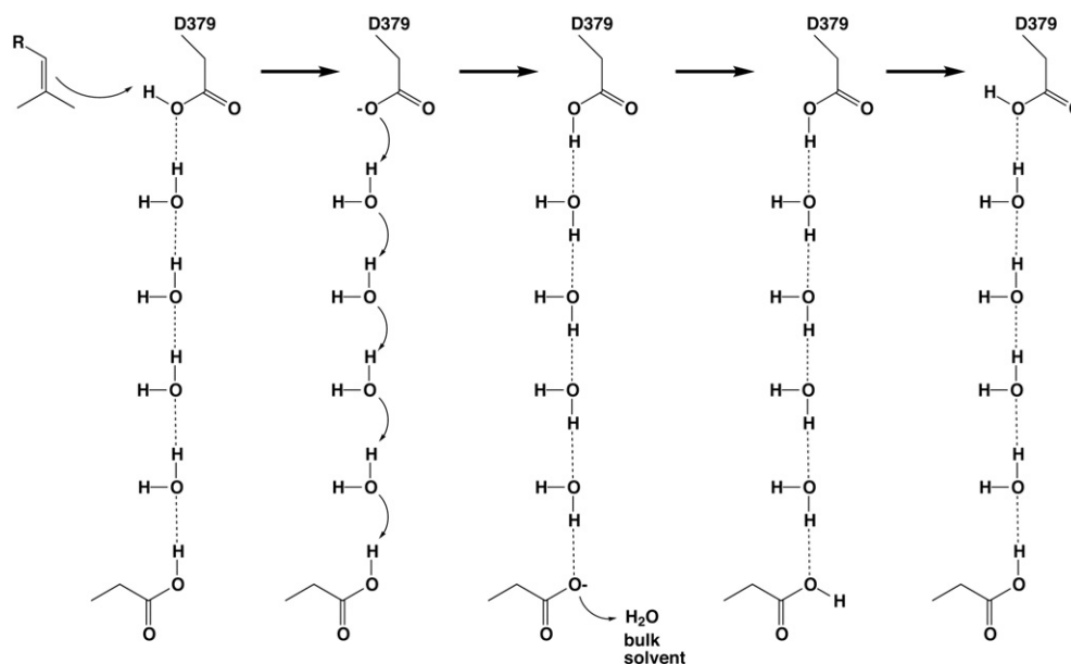
Fig. 5. General acid D379 could be reprotonated by Grotthuss diffusion of a proton across a 4-solvent “proton wire” in a polar channel leading to another aspartic acid serving as a proton shuttle to bulk solvent, such as D503 or D336; in order for D336 to serve in this capacity, its hydrogen bond with R340 must be displaced by a solvent molecule.
