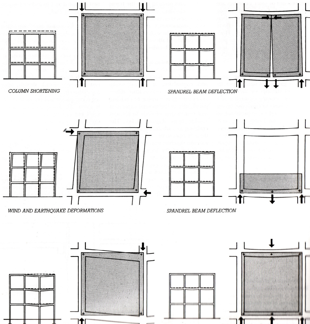
Figure 2.12. Alternative deformation of cladding components depending on building movement (Source: Brock 2005).
