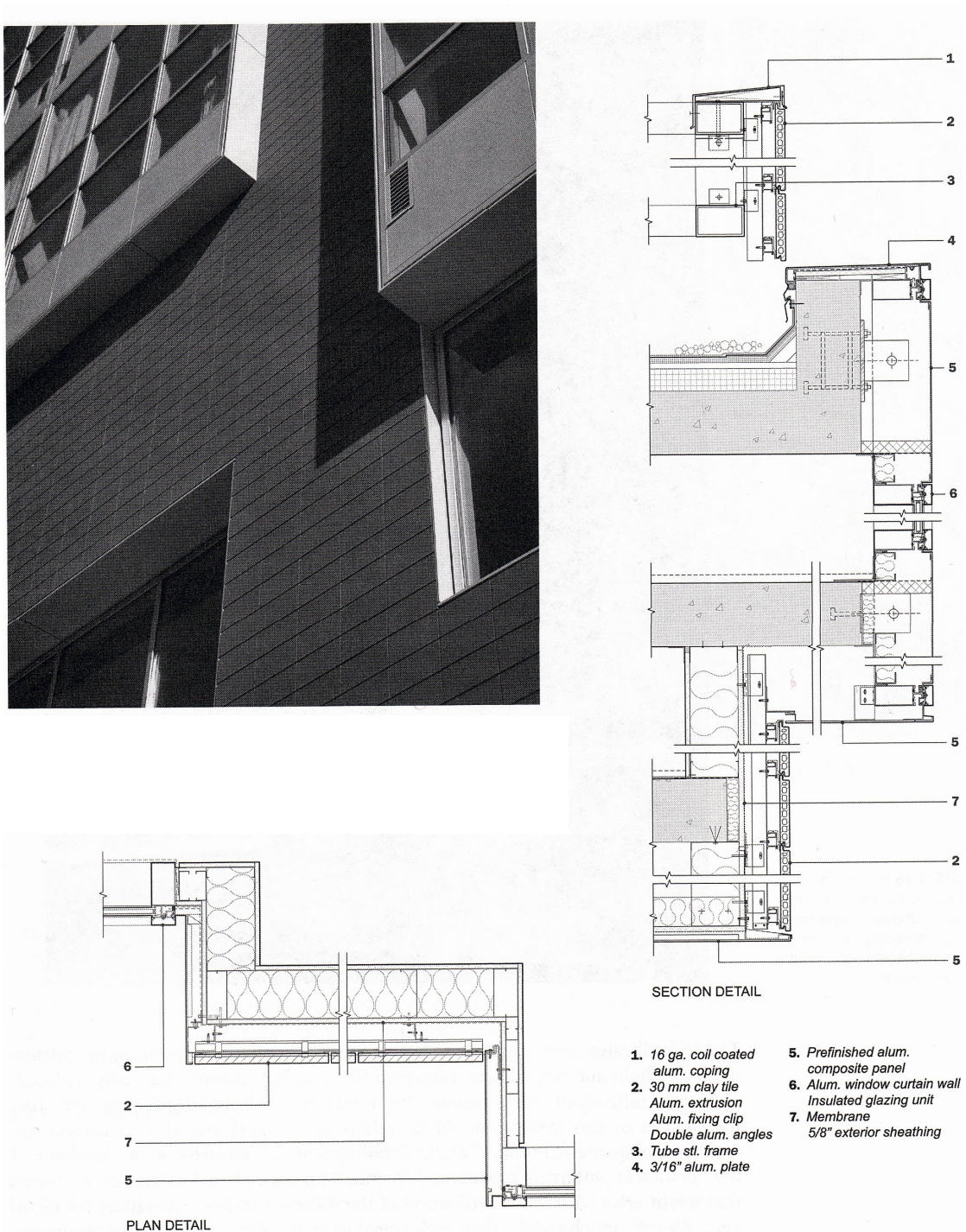
Figure 2.23. Details of terra-cotta tile cladding (Source: Allen 2004)
