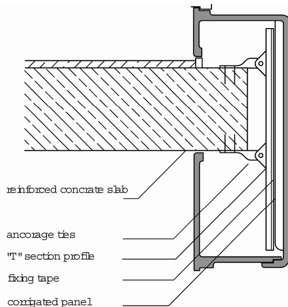
Figure 4.9. Fixing detail
