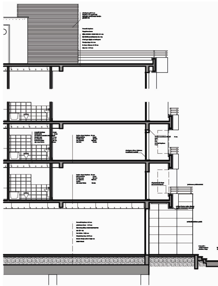
Figure 4.8. Partial section
