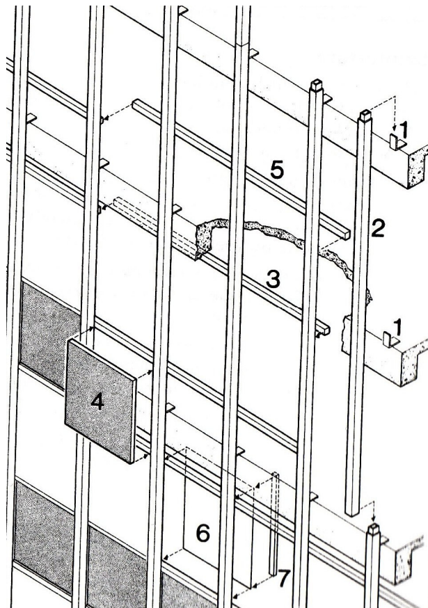
Figure 2.13. Schematic drawing of typical version of stick System (Source: Brock 2005).
