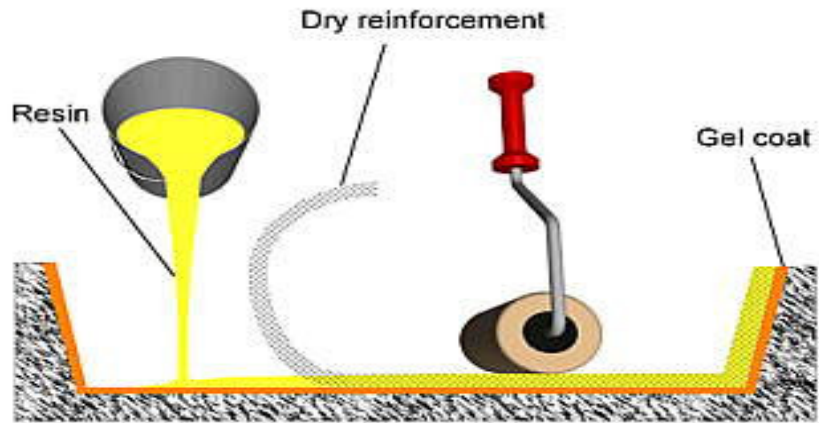
Figure 4.16. Hand lay-up methods
