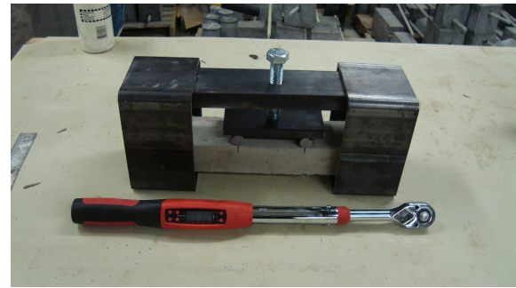
Fig. 3 Four-point sustained flexural loading test set-up.
