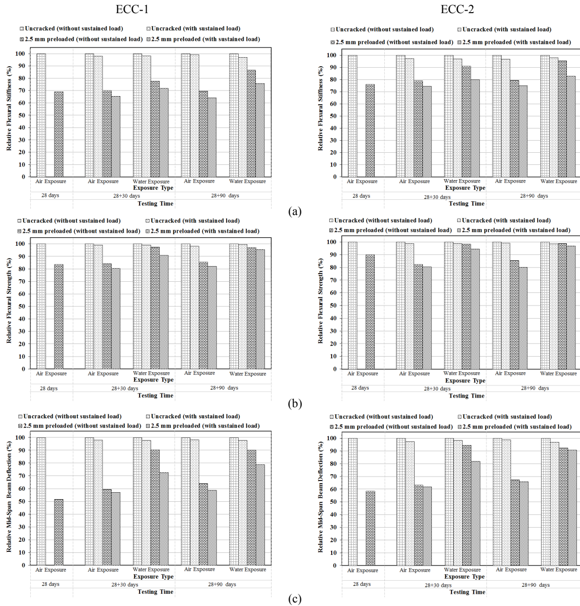
Fig. 6 Influence of different exposure regimes and sustained mechanical loading on mechanical properties of ECC mixtures: (a) Flexural stiffness, (b) Flexural strength, and (c) Flexural deformation capacity.
