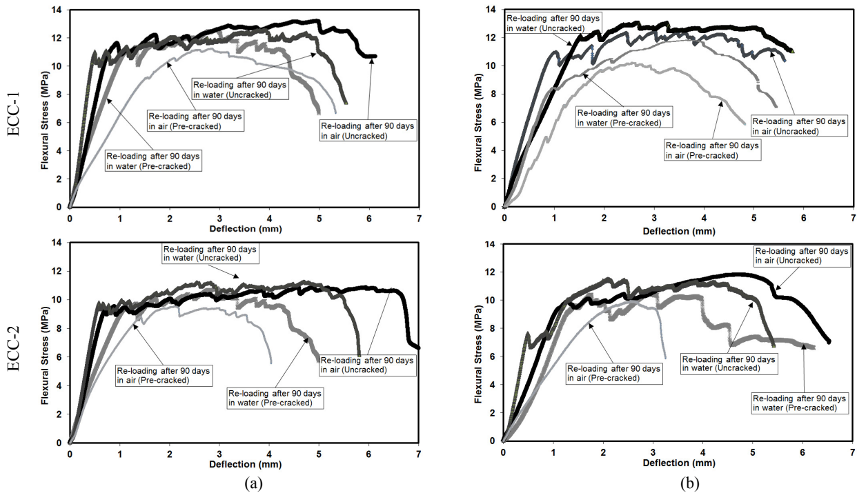
Fig. 5 Effects of different exposure and loading conditions on flexural stress-displacement behavior of ECC mixtures: (a) without and (b) with sustained mechanical loading.
