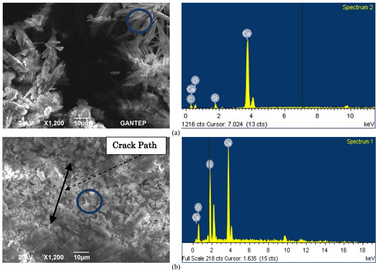
Fig. 8 SEM micrograph with EDX pattern of rehydration products in a self-healed crack of ECC-1 specimen: After (a) 30 days, and (b) 90 days wet exposure.
