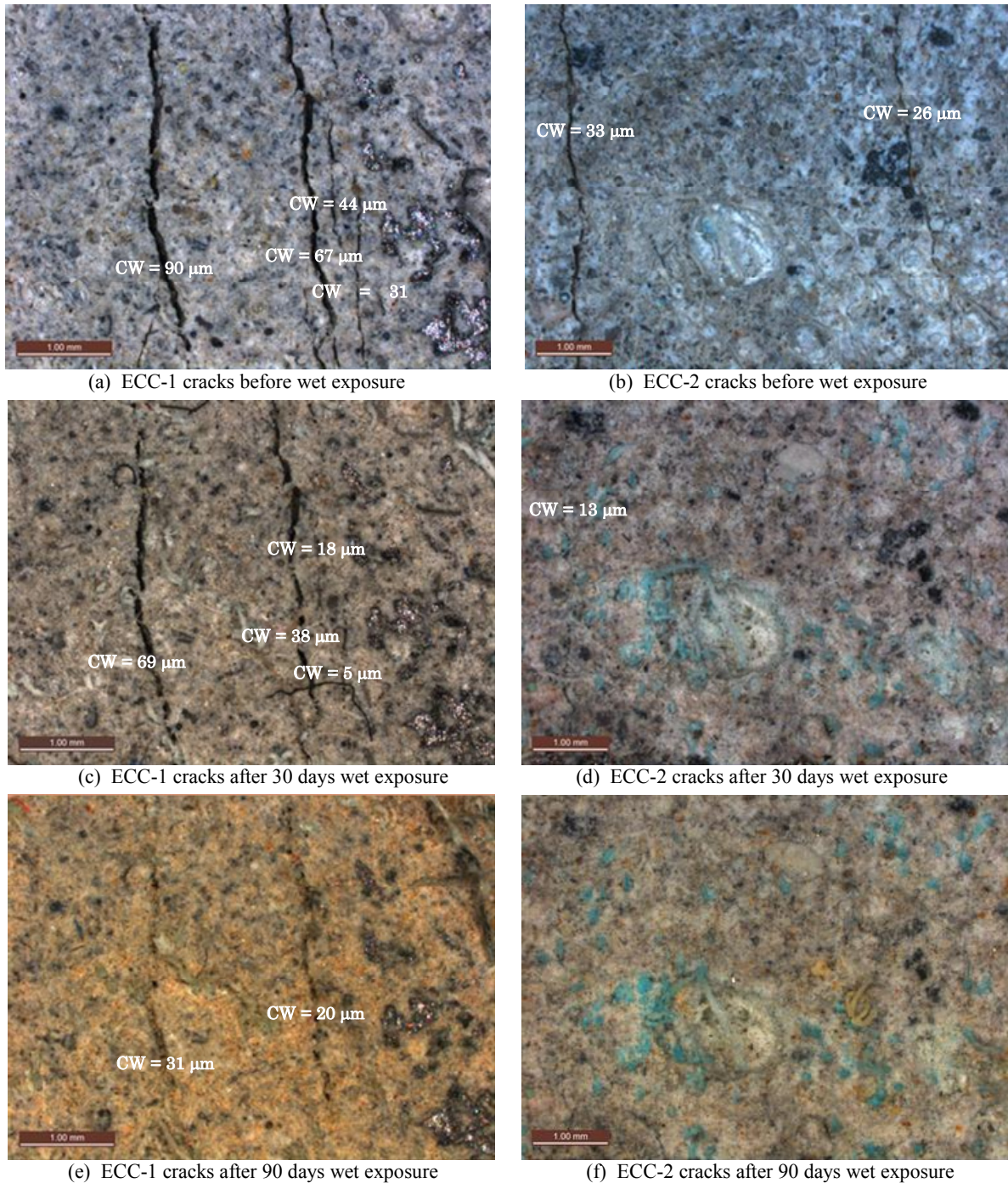
Fig. 7 Self-healing products in ECC microcracks before and after continuous water exposure.
