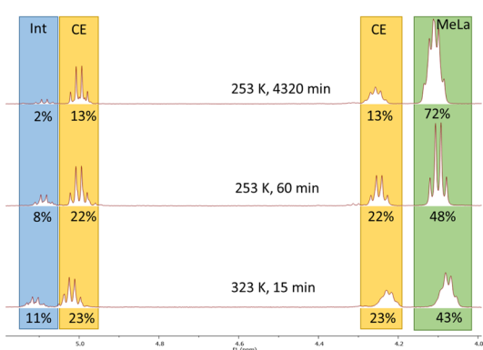
Figure 8. ^1\text{H} NMR ( \text{C}_6\text{D}_6 , 400 MHz) stacked spectra and corresponding concentrations from the \text{Zn}(\text{2}^{\text{Pr}})_2 degradation tests at 253.2 K.
