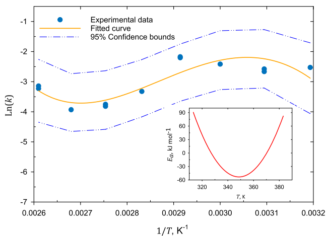
Figure 6. Curved Arrhenius plot for the rate coefficient of the degradation step and corresponding variable activation energy (inset) given by eq 16.
