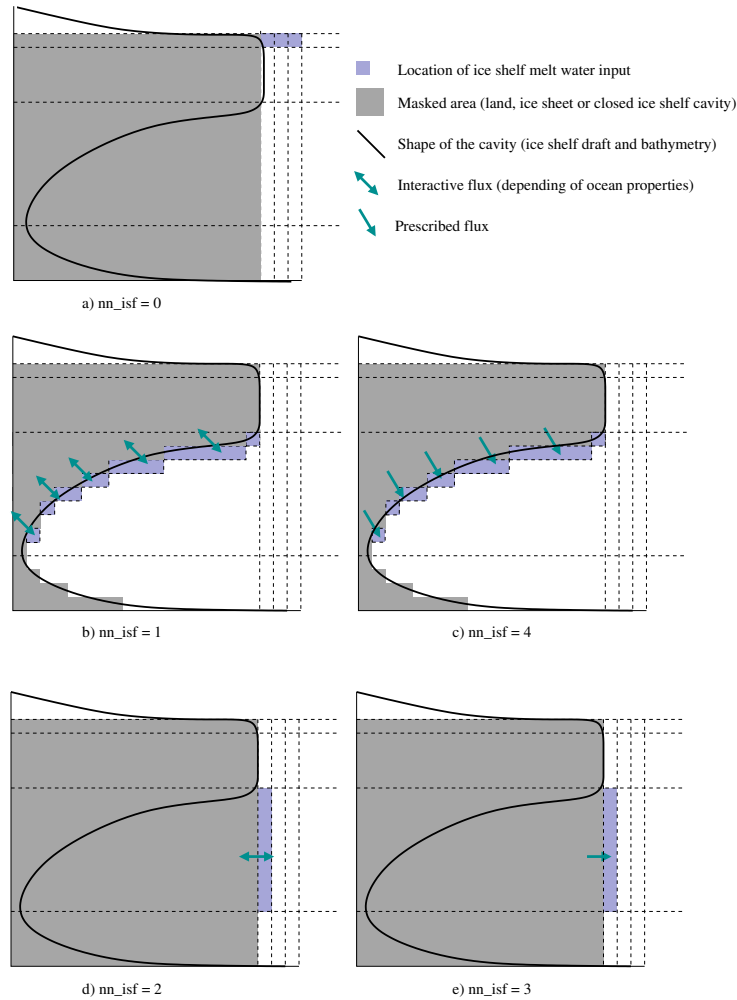
Figure 7.1: Schematic for all the options available through nn_isf .
