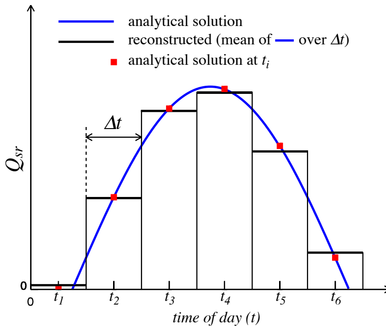
Figure 7.2: Example of reconstruction of the diurnal cycle variation of short wave flux from daily mean values. The reconstructed diurnal cycle (black line) is chosen as the mean value of the analytical cycle (blue line) over a time step, not as the mid time step value of the analytically cycle (red square). From Bernie et al. [2007] .
