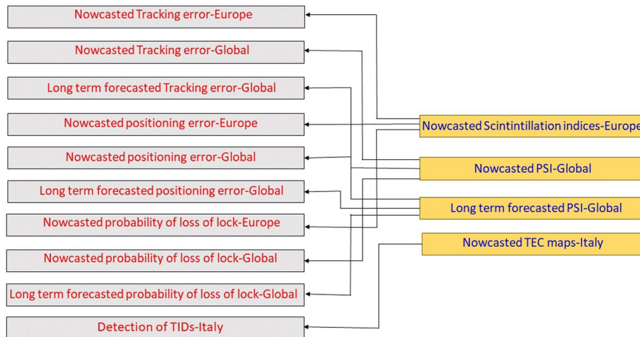
Fig. 4. Scheme reporting the input data types for the RPF-3 algorithms.
