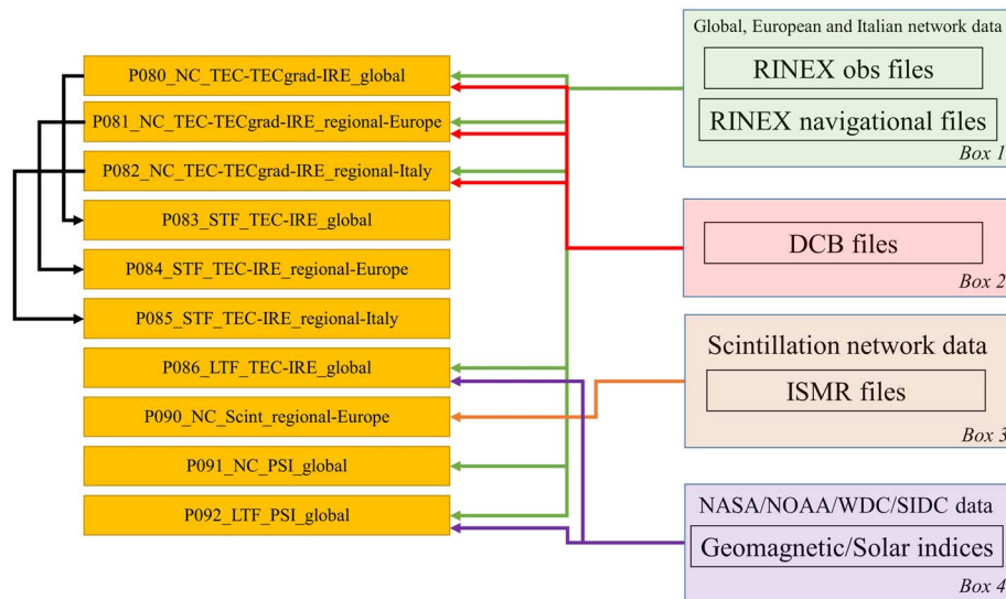
Fig. 2. Block diagram summarizing the RPF 2 products and their input data.
