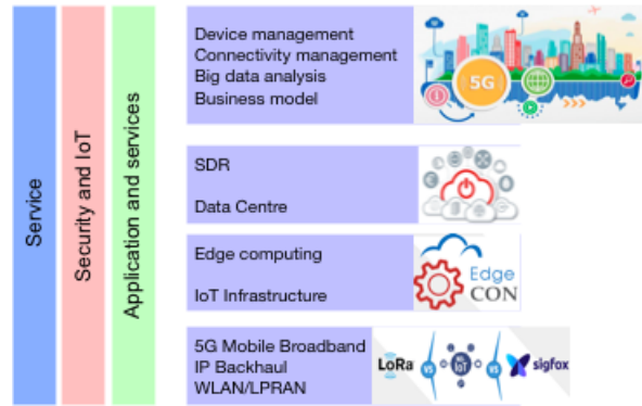
Figure 5: Architecture
