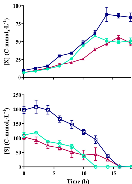
Figure 2. Heterotrophic biomass production (dark) and substrate consumption (open) of C. sorokiniana SAG 211/8K cultivated in M8a medium with 100 \text{C} \cdot \text{mmol}_s \cdot \text{L}^{-1} sodium acetate (circles), 200 \text{C} \cdot \text{mmol}_s \cdot \text{L}^{-1} sodium acetate (squares), and 100 \text{C} \cdot \text{mmol}_s \cdot \text{L}^{-1} glucose (triangles).
