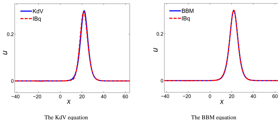
Fig. 1. The solitary wave solution of the unidirectional wave equation (solid line) and the corresponding approximate solution of the IBq equation (dashed line) at t = 20 .
