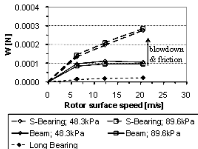
Figure 9: Comparison of the lift force estimates by long and short bearing theories with beam theory deflection force calculations [10].
