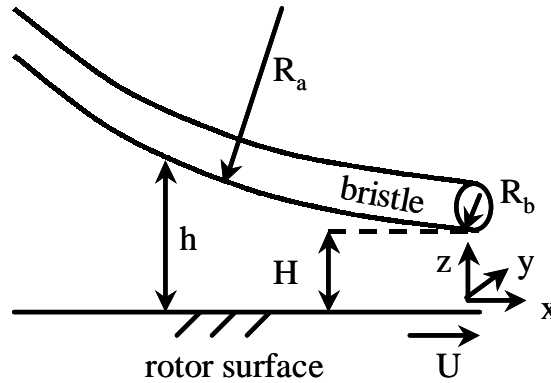
Figure 7: Hydrodynamic lift geometry for bristles [8].
