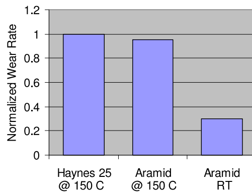
Figure 3: Wear test results for aramid and Haynes 25 tufts against Ni-Cr-Mo-V. Data are normalized with wear rate of Haynes 25 bristles at 150 °C [6].
