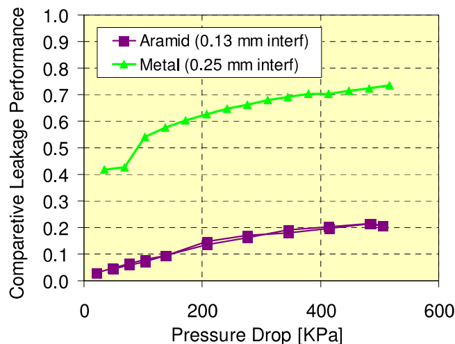
Figure 5: Comparison of leakage rates of aramid and metallic brush seals [6].
