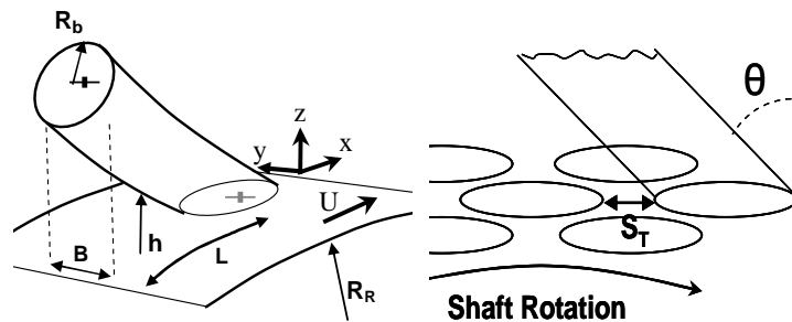
Figure 8: Bristle spacing ( S_T ) characterizes oil lift region at bristle tips. [9].
