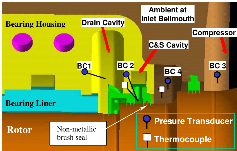
Figure 2: The 7EA gas turbine inlet bearing brush seal application [6].
