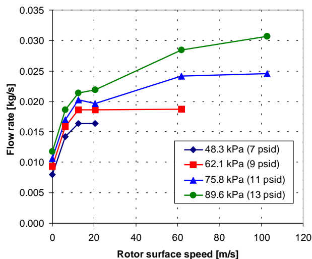
Figure 6: Hydrodynamic lift of brush seals with rotor speed [7].
