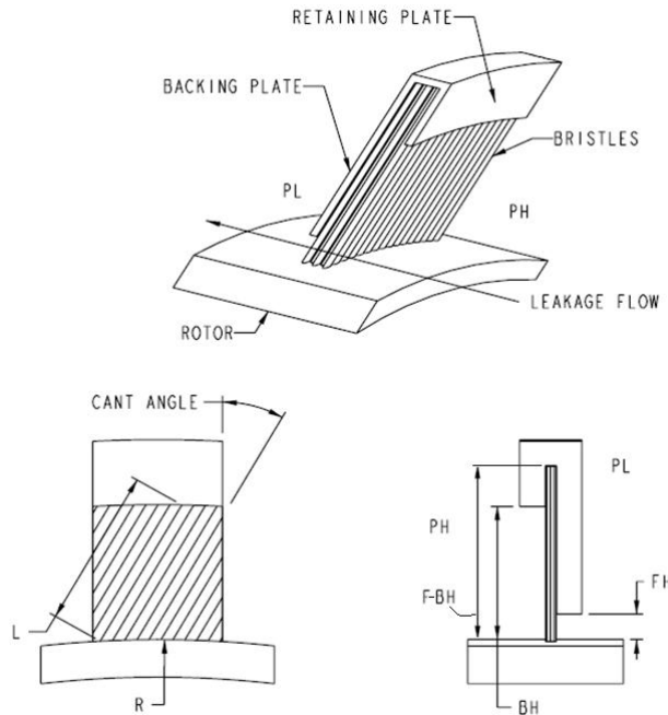
Figure 1: Brush seal schematic and main design parameters.
