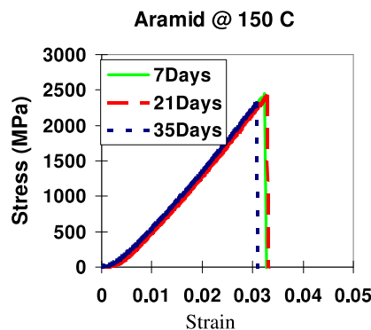
Figure 4: Aramid fiber strength upon exposure to 150 °C (300 °F) [6].
