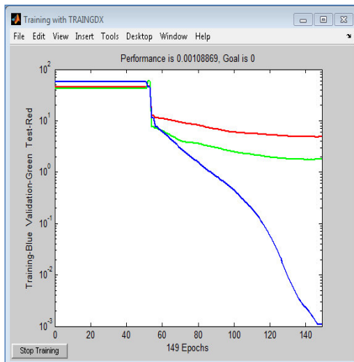
Figure 7: Training result for the ideal BP NN with 300 hidden nodes and Log sigmoid activation function
