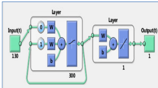
Figure 12: The ideal RNN architecture
