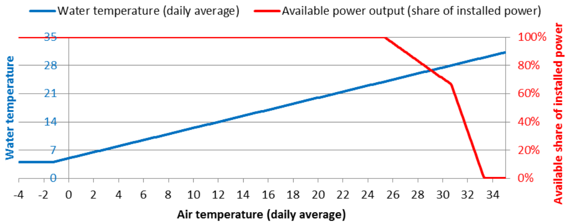
Figure 13: Availability constraints on thermal plant output linked to air and water temperatures
