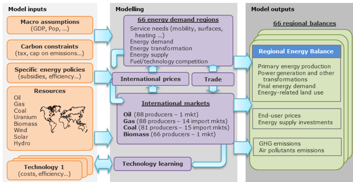
Figure 11: POLES model general scheme
