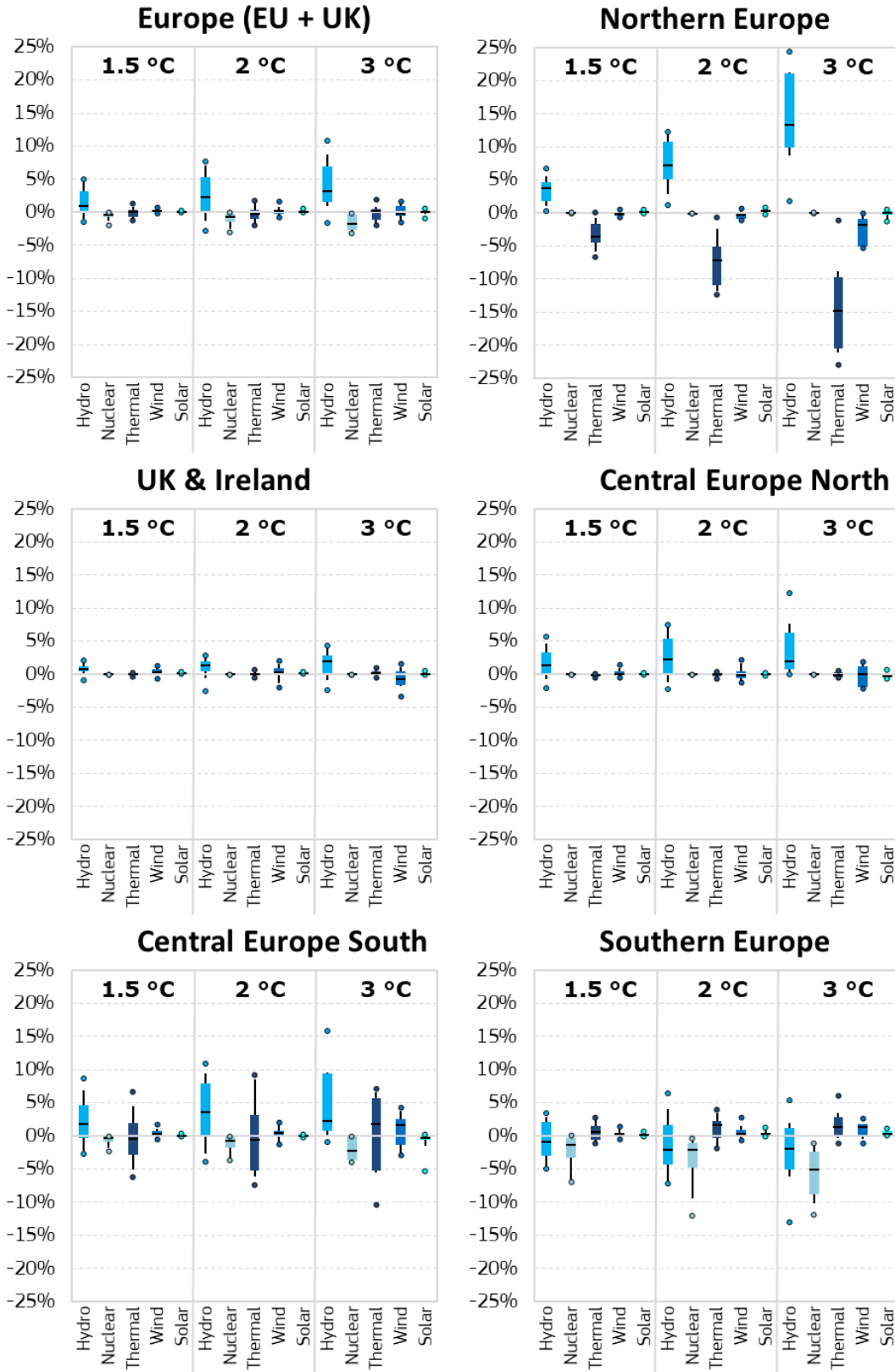
Figure 2: Climate change impacts on 2020's electricity production by energy source in Europe, by region To read the figure, note that "thermal" designates biomass, coal, gas and oil plants' production. The scenarios represented are based on 11 climate models, with RCP 4.5 (compatible with 1.5 and 2 degree warming levels) and RCP 8.5 (used for 1.5, 2 and 3 degree warming levels). Dots indicate the extreme scenarios; vertical lines indicate the spread of all other points; coloured areas indicate the two middle quartiles separated by the median line. All effects other than climate impact on electricity supply are neutralized; only the relative differences of production of each electricity source are shown.
