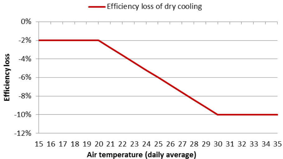
Figure 14: Efficiency losses of thermal plants due to dry cooling
