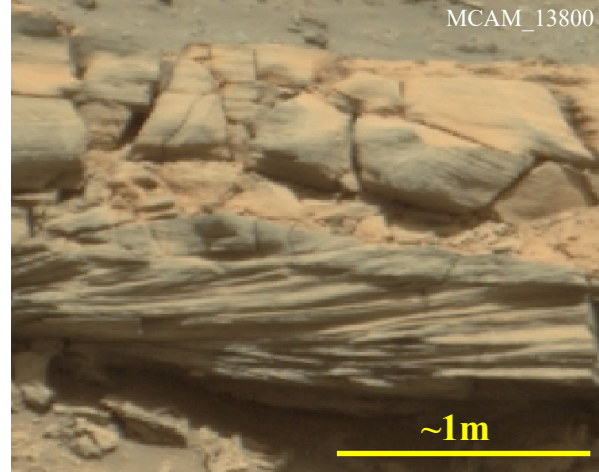
Fig. 4: Mastcam image of the pediment capping unit near Tower butte (Fig.1) showing undulating lower contact and 0.5m scale cross-stratification.
