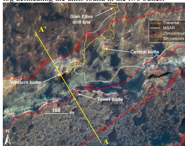
Fig. 1: map with cross-section for Fig 5.
