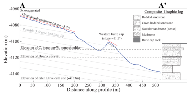
Fig. 3: cross-section A-A' (Fig. 1) with composite graphic log of facies correlated across the two buttes.
