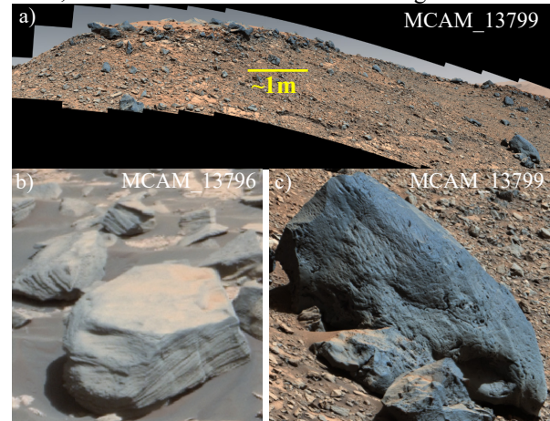
Fig. 5: a) Mastcam image of the capping unit at Western butte (Fig.1). b) block of fallen pediment near Tower butte (Fig. 1). c) block of fallen Western butte cap. Note: b and c are both roughly meter-scale boulders.
