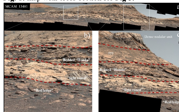
Fig. 2a-c: Mastcam images of Central butte indicating approximate stratal boundaries. Note butte is ~10m tall
