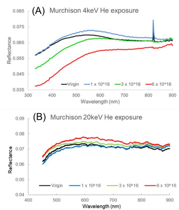
Fig. 1. Reflectance spectra of Murchison CM chondrite irradiated by 4keV He (A) and 20keV He (B) with total dose of 1, 3, \text{ and } 6 \times 10^{16} ions/cm 2 .
