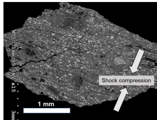
Fig. 2. Back-scattered electron image of MET01072 CM chondrite, showing high densities of parallel fractures in a direction perpendicular to the shock compression axis.
