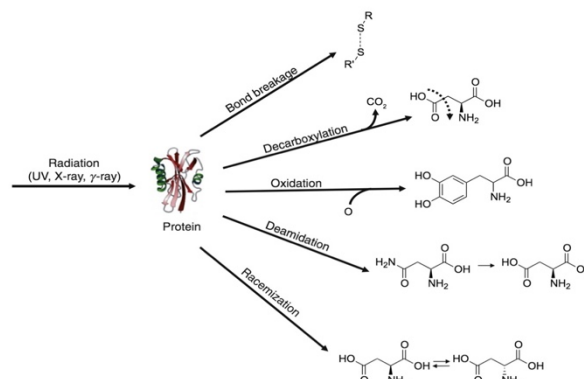
Figure 2: Examples of the types of alteration that organic compounds may experience as a result of primary and secondary effects following X-ray exposure. Image from [6].
