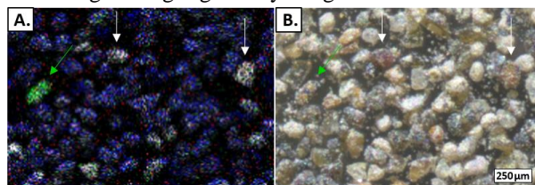
Figure 4: A. Micro-XRF compositional map of sediment sample. Red=Cr, green=Mn, gray=Fe, blue=Ca. B. Corresponding microscope image.
