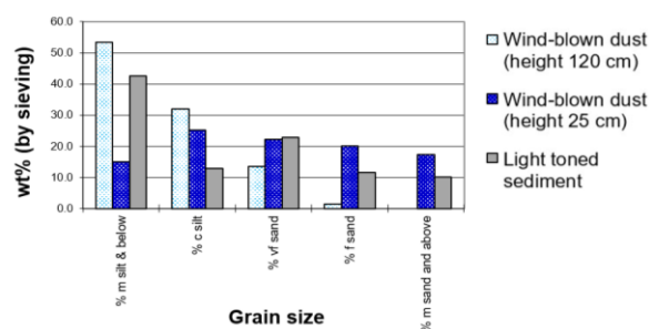
Figure 2: Grain-size distribution of two wind-blown dust samples and one sample of local ground sediment.
