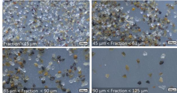
Figure 3: Microscope images of 4 grain-size separates, from wind-blown dust collected at height=120cm.
