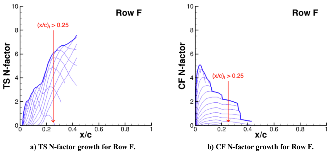
Figure 31. N-factor growth for crossflow (CF) and Tollmien-Schlichting (TS) at outboard Row F. The vertical red marker is the approximated transition location from the corresponding TSP image. The test conditions are M = 0.86 , T_T = -50 \text{ }^\circ\text{F} , \alpha = 2.5 \text{ deg.} , and Re_{MAC} = 17.5 \text{ million} .
