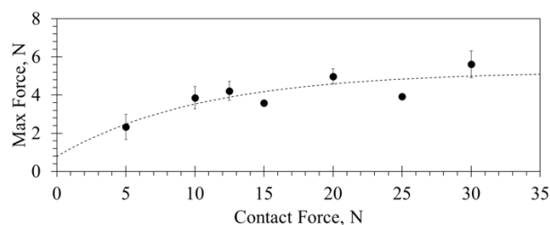
Figure 3. Tack force increased as the probe compaction force increased. Temperature, humidity, and dwell time were all constant at 40 °C, 40%, and 5 s, respectively.
