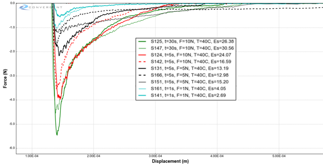
Figure 9 Test data from DOE 2 of the decohesion segment with varying contact time (t) and applied contact force (F) for a given temperature (T) including the calculated Energy of Separation (Es) for an individual sample (S).
