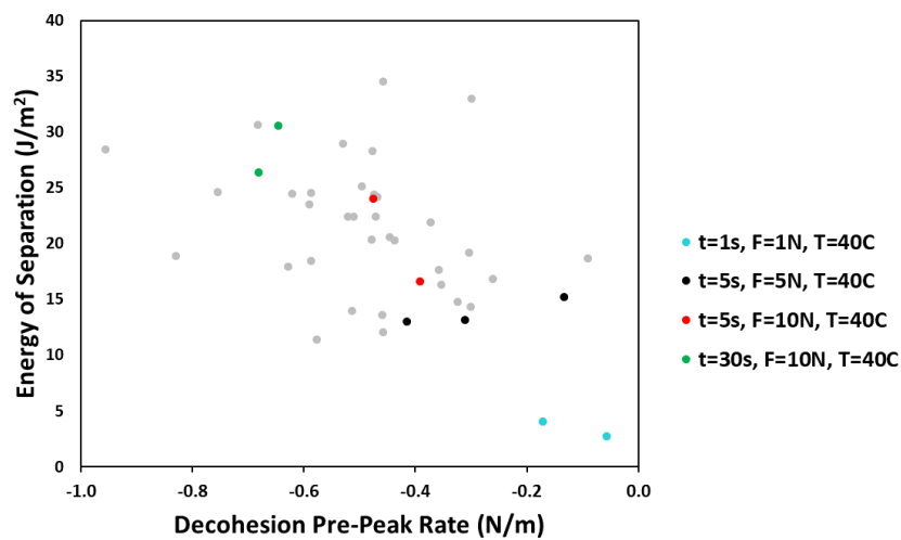
Figure 10 Energy of separation as a function of the rate at which the force reaches the decohesion peak for varying contact time (t), applied contact force (F), and temperature (T) corresponding to the test data in Figure 9
