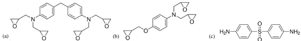
Figure 2: Structures of (a) the tetrafunctional epoxy, 4,4'-methylenebis(N,N-diglycidylaniline), (b) the trifunctional epoxy, N,N-diglycidyl-4-glycidyoxyaniline, and (c) the tetrafunctional hardener 4,4'-diaminodiphenyl sulfone (DDS).
