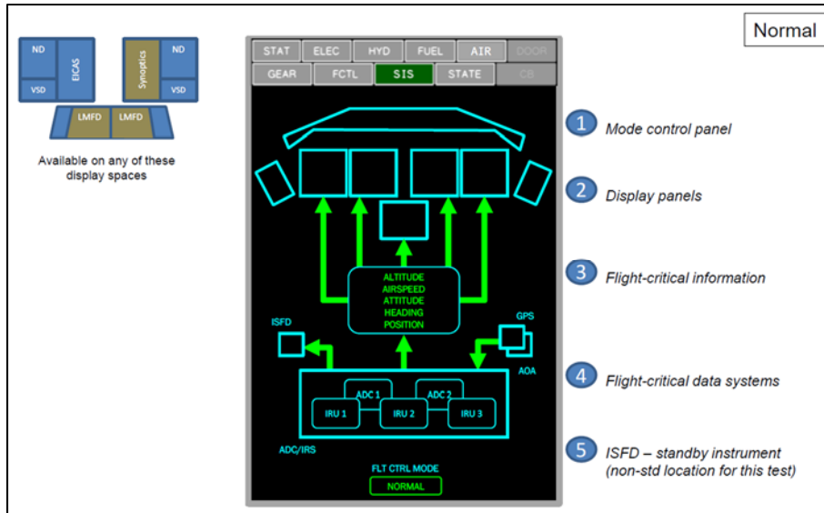
Fig. 1. SIS indicators and functions on the synoptic display (normal conditions).
