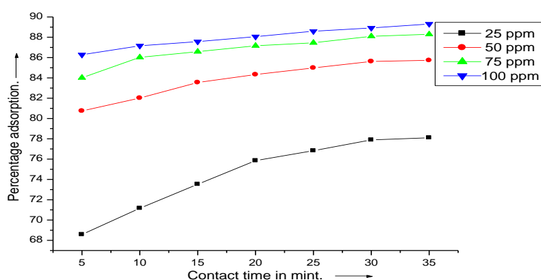
Fig.2: Effect of contact time and initial concentration of CV dye on adsorption of RGSH adsorbent. [Adsorbent dose=1.0 gm., Volume=50 ml., Temp.=300.8 K, pH=7.2]
