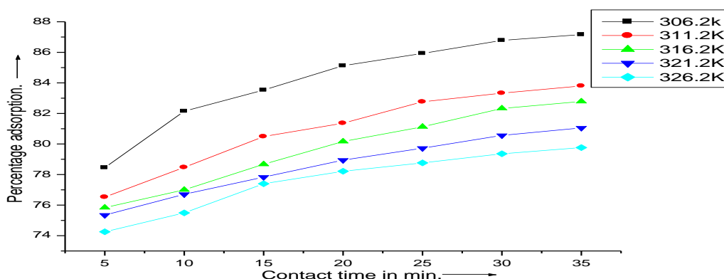
Fig.4: Effect of temperature on CV dye adsorption on RGSH adsorbent. [adsorbent dose=1 gm., Int. conc.=50 ppm., Volume=50 ml, pH=7.2.]
