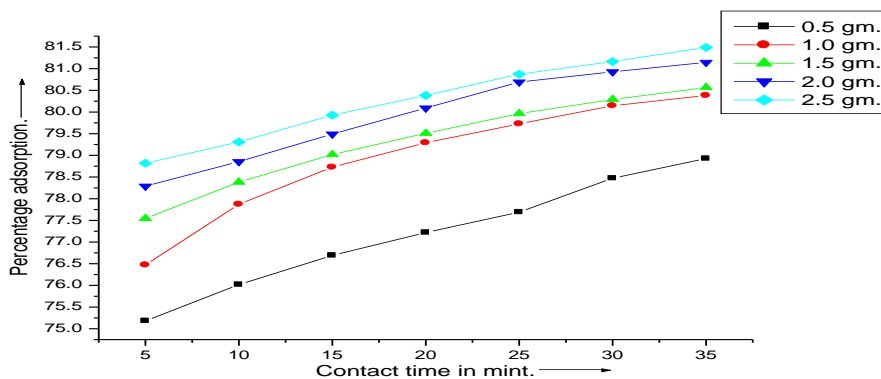
Fig.3: Effect of adsorbent dose of RGSH on adsorption of CV dye. [Initial conc.= 50 ppm, Volume of adsorbate=50 ml, Temp.=300.8K, pH=7.2]
