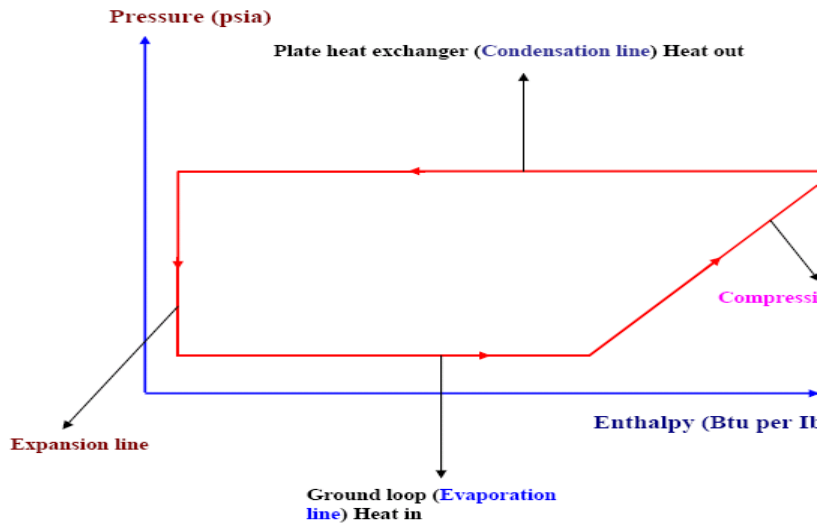
Figure 12. The ideal cycle on Pressure-Enthalpy diagram.
