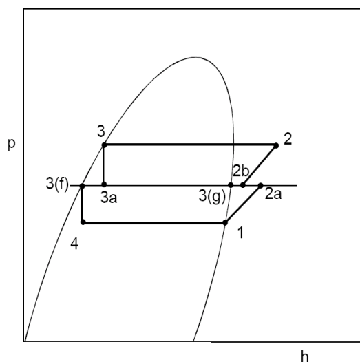
Figure 21. Cycle of multiple compressions using flash chamber.
