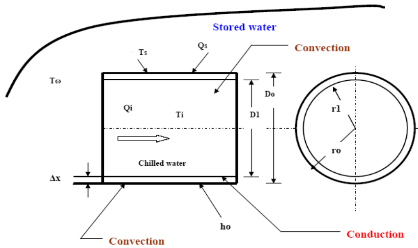
Figure 11. Schematic of heat transfer through a circular tube heat exchanger.
