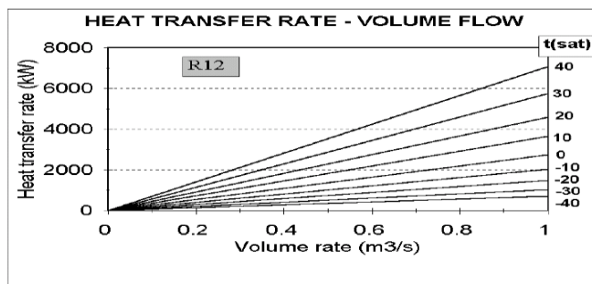
Figure 5. Heat transfer rate versus volume rate.
