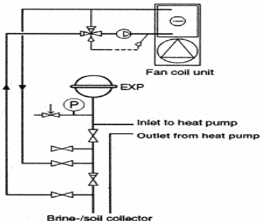
Figure 3. Diagram of cooling system.
