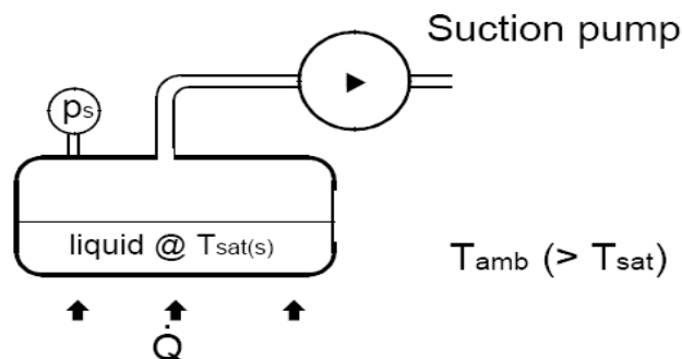
Figure 4. Refrigeration Cycle.
