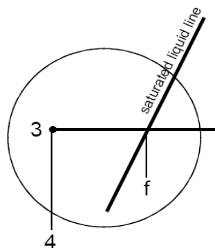
Figure 17. Condenser sub-cooling.
