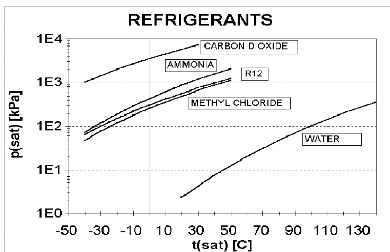
Figure 9. Refrigerant chart.
