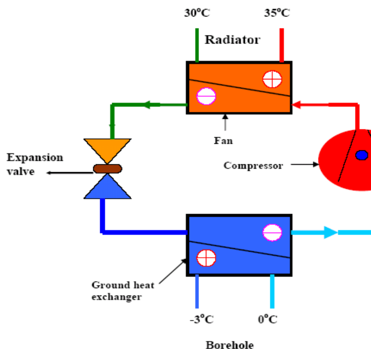
Figure 2. Detail of the GSHP circuit.
