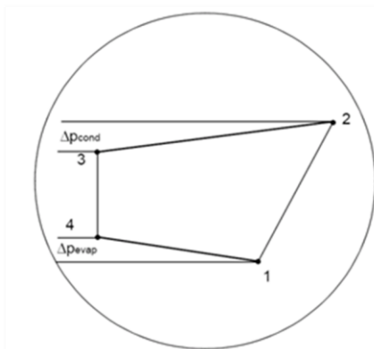
Figure 18. Pressure drops in evaporator and condenser.
