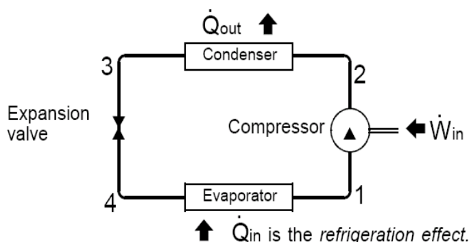
Figure 7. Simplified refrigeration system diagram.
