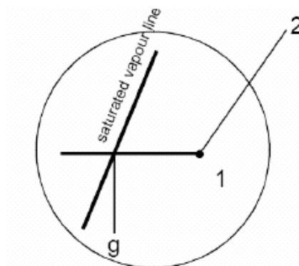
Figure 15. Evaporator superheat.
