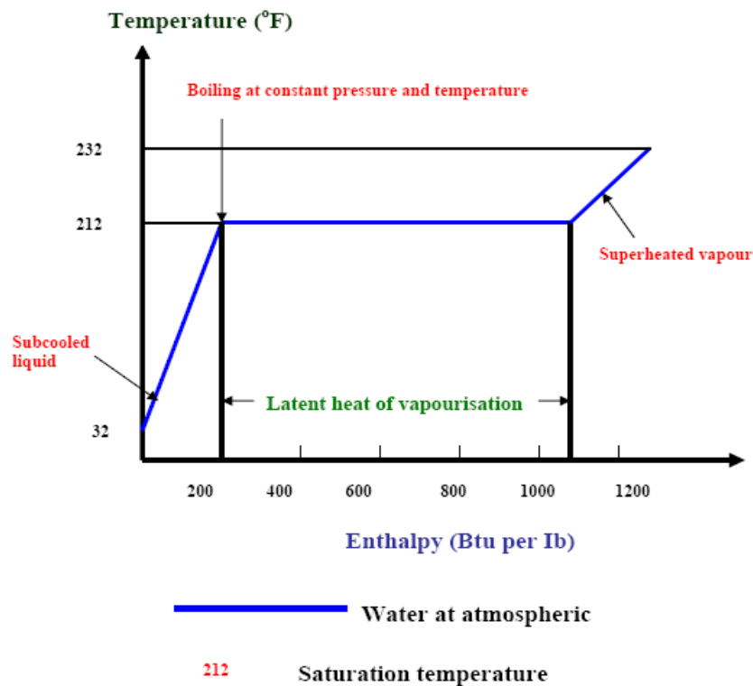
Figur 13. Water undergoing a charge of state.
