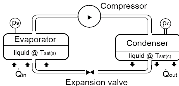
Figure 8. Heat pump refrigeration cycle.
