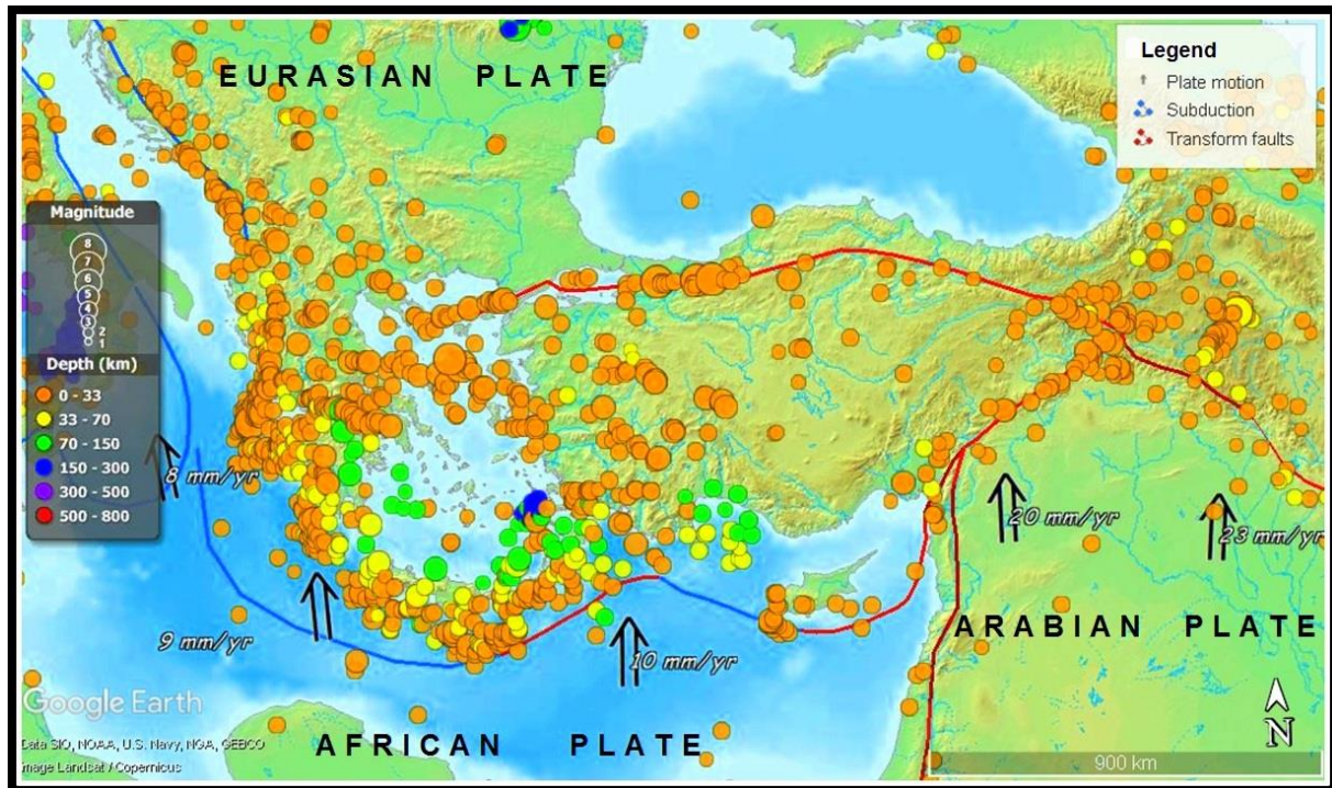
Fig.4: Main tectonic processes (subduction, faulting, earthquakes – circles on the figure) in the Eastern Mediterranean region (GIS data: [26])
