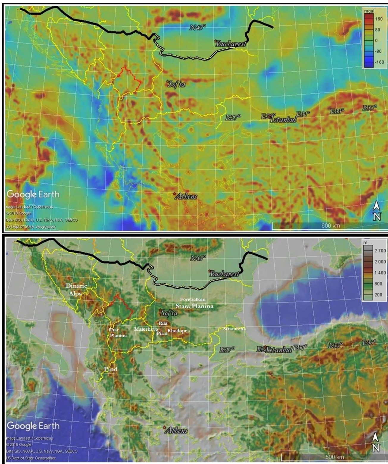
Fig.3: Correlation between positive Free-Air gravity anomalies (above) and DEM (below) within the Balkan Peninsula
