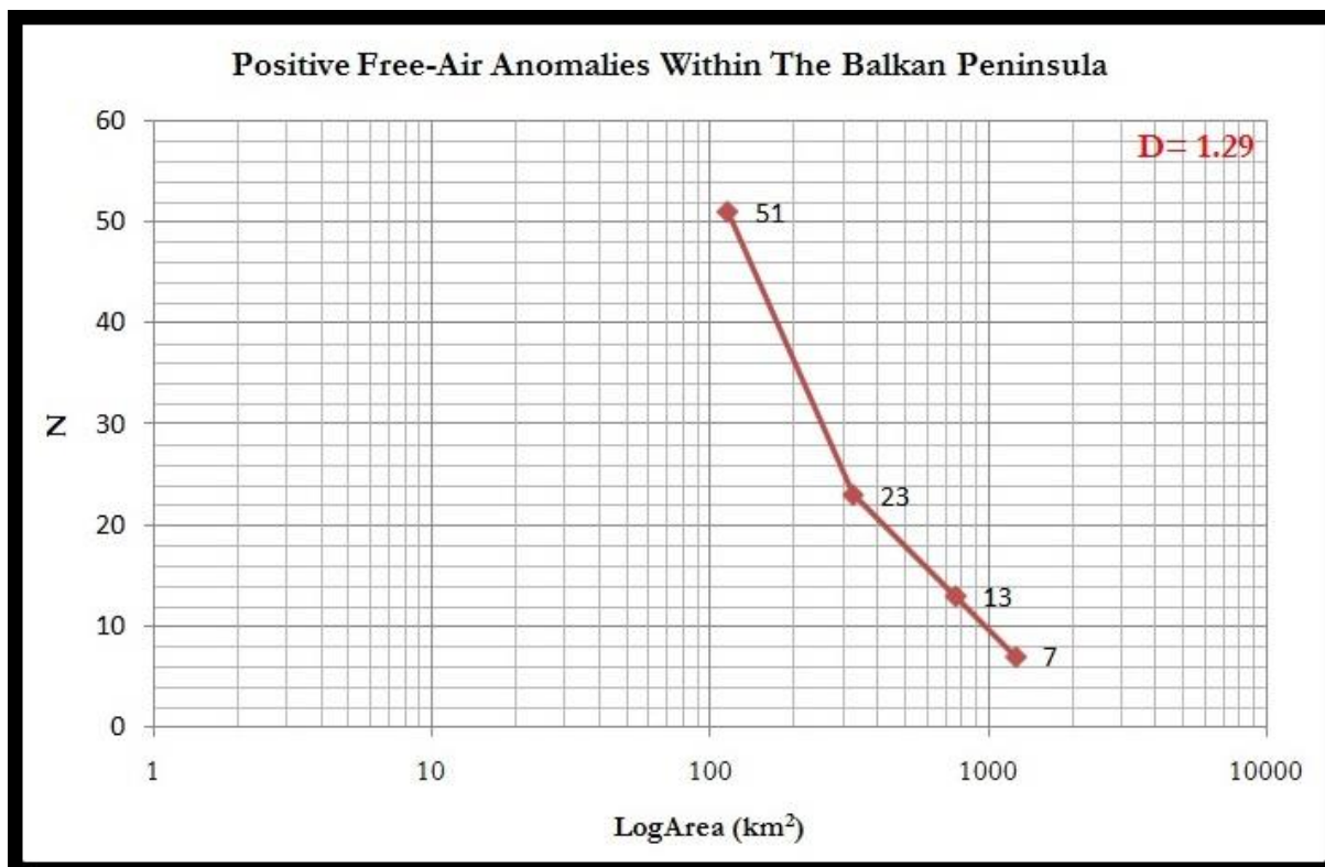
Fig.5: Fractal diagram of the positive Free-Air gravity anomalies within the Balkan Peninsula
