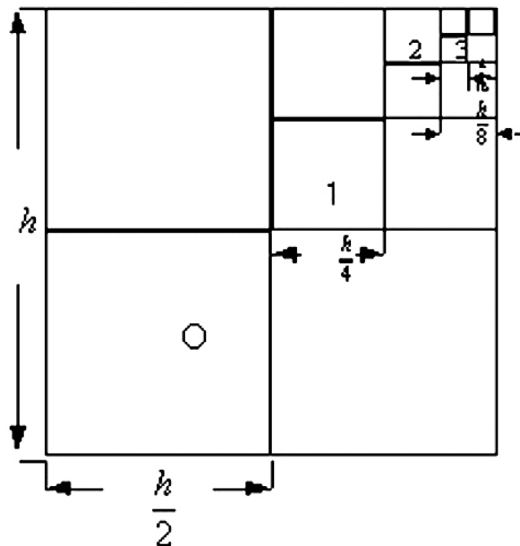
Fig.2: 2D fractal scheme – each linear element is 1/2 of the larger one.
