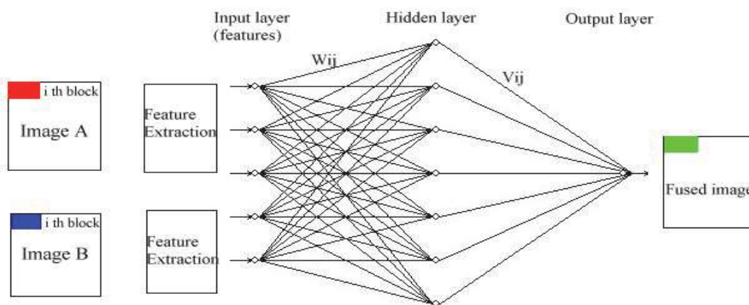
Figure 11. Schema of the ANN-based image fusion method [24]
