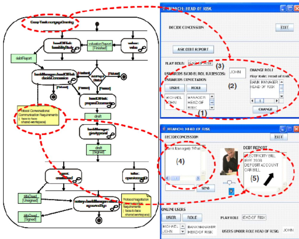
Figure 2. Mapping of cooperative task and interaction protocols to groupware components (Rodríguez et al., 2007).
