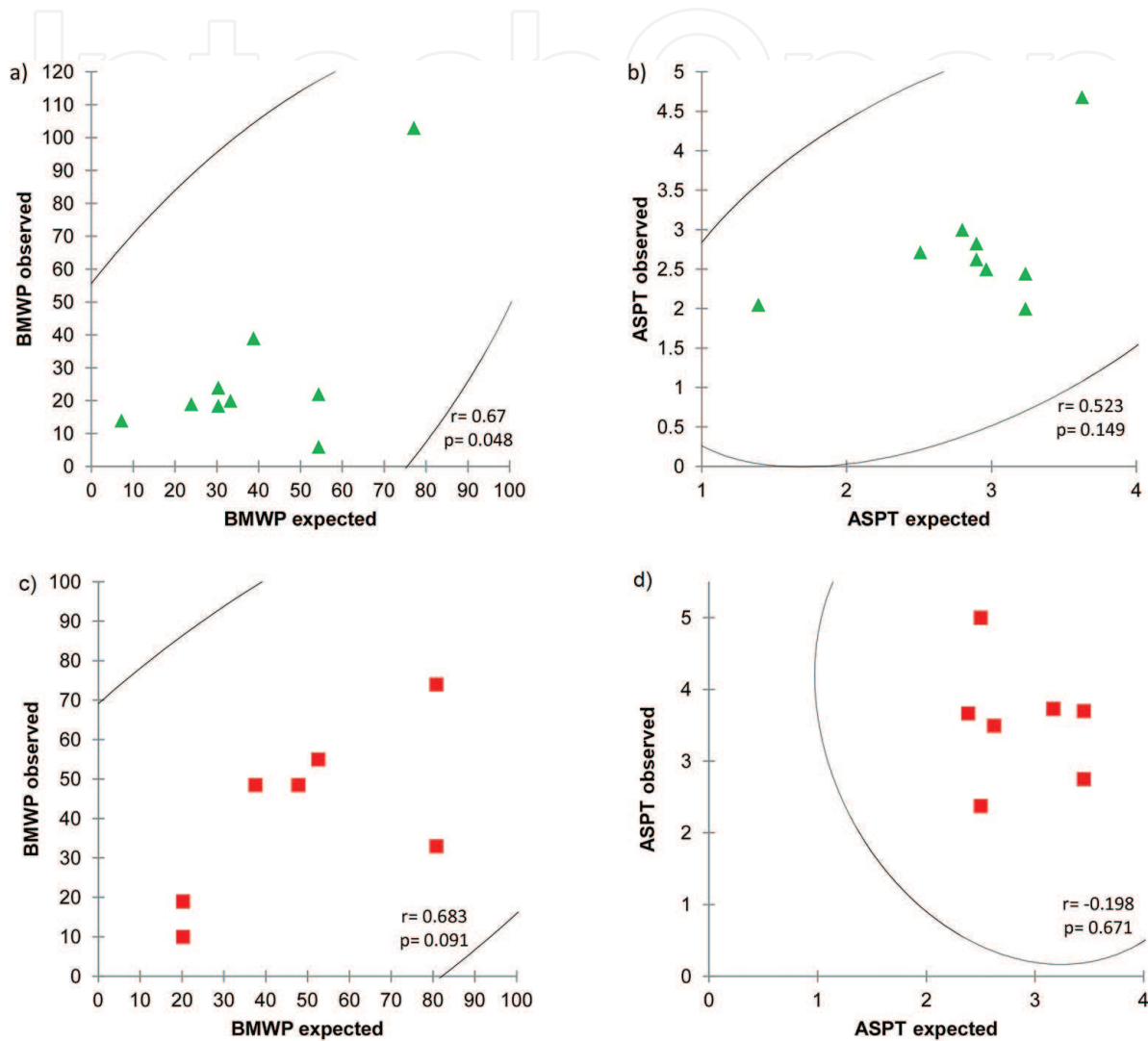
Figure 6. Validation and range extension data correlation. (a) Validation BMWP observed vs expected. (b) Validation ASP observed vs expected. (c) Extension BMWP observed vs expected. (d) Extension ASP observed vs expected.
