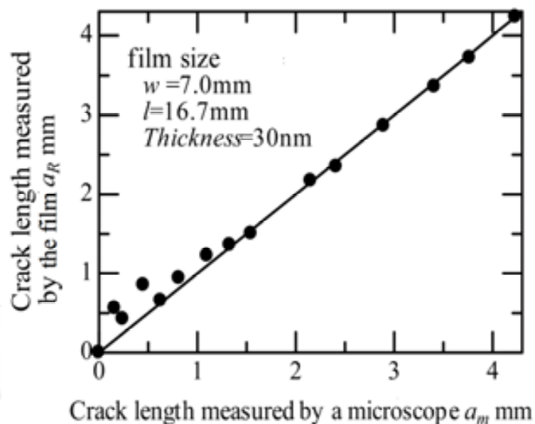
Fig. 13. Comparison of crack length obtained by microscope and ion-sputtered film
