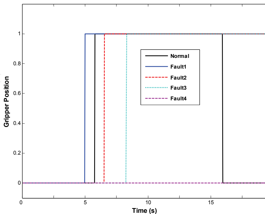
Fig. 4. Gripper Pick
