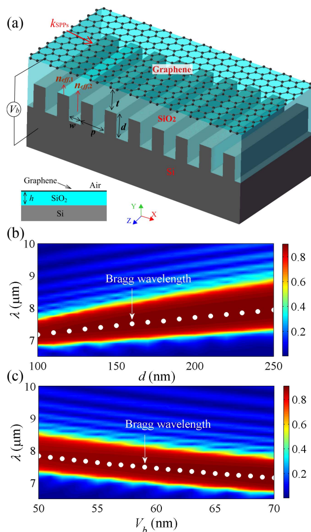
Figure 1 | Schematic and reflectivity of the graphene Bragg grating. (a) Schematic illustration of the graphene-based plasmonic Bragg grating structure. The surface conductivity of the graphene monolayer on silica (SiO 2 ) can be tuned through an external gate voltage ( V_b ). The silicon (Si) substrate has a groove grating structure with period p , width w and depth d . t denotes the distance between the graphene and Si substrate. The inset shows a basic graphene-SiO 2 -Si structure with a SiO 2 layer thickness h . (b) shows the reflectivity as a function of wavelength \lambda and grating groove depth d for a constant voltage V_b = 60 \text{ V} and (c) as a function of wavelength \lambda and applied gate voltage V_b for a constant depth d = 150 \text{ nm} . The other parameters are set as t = 100 \text{ nm} , p = 2w = 40 \text{ nm} , T = 300 \text{ K} and \mu = 20000 \text{ cm}^2\text{V}^{-1}\text{s}^{-1} . In the FEM simulations, the number of grating periods is 16 and SPP modes in graphene are excited from the left as indicated by the red arrow. The white circles represent the theoretical results for the Bragg grating operating wavelength obtained by solving Eq. (5).
