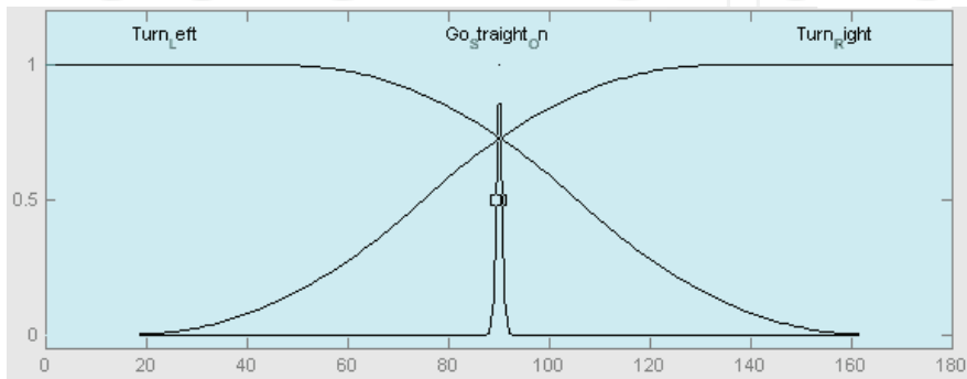
Fig. 7. Typical output variable membership function plot.
