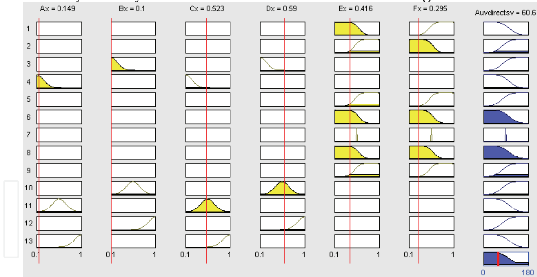
Fig. 8 Rule viewer for fuzzy controller.
