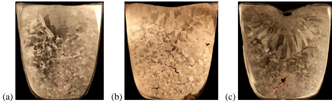
Figure 2. The macroscopic grain structure of the samples: (a) without UT, (b) range I with UT until just before solidification begins in the temperature range 714-660°C, and (c) range V with UT applied for 4 minutes starting at 655°C.
