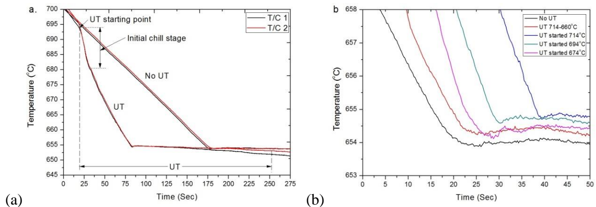
Figure 4. Cooling curves: (a) with and without UT and (b) cooling curves focused on the nucleation stage from thermocouple 2 (T/C2) indicated in Figure 1a.
